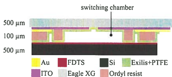
Figure 4: Schematic layer structure of the fluidic chip.
