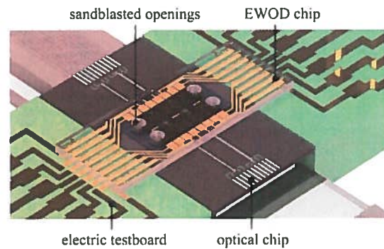
Figure 3: Rendered 3D-Model of the chip assembly.
