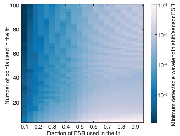
Figure 3: Minimum detectable wavelength shift of Vernier sensor per FSR in function of fraction of the FSR used and number of points used in fit.
