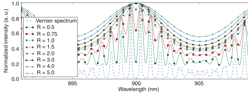
Figure 5: Convolution of Vernier spectrum with Gaussian channels of different width. R indicates the ratio of the filter channel width to the period of the constituent Vernier peaks.
