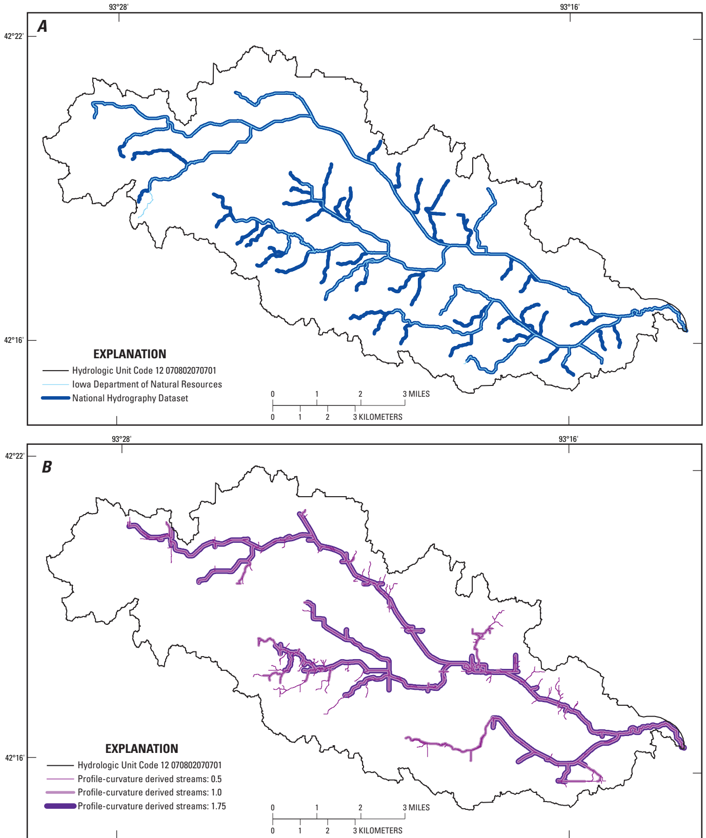
Figure 3. Examples of derived streams for hydrologic unit code 12 070802070701 (0545129280, Honey Creek Tributary near Radcliffe, Iowa, site 5 in figure 1) from initiation methods based on A , the National Hydrography Dataset and the Iowa Department of Natural Resources and B , three thresholds of profile curvature and requirements for continuity.
