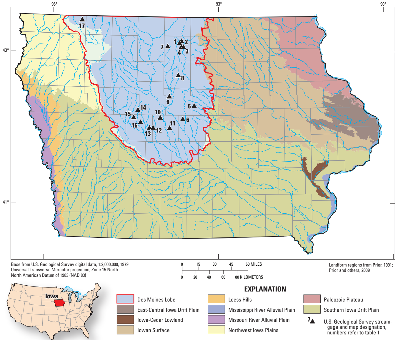
Figure 1. Des Moines Lobe landform region and U.S. Geological Survey streamgages included in this study.
