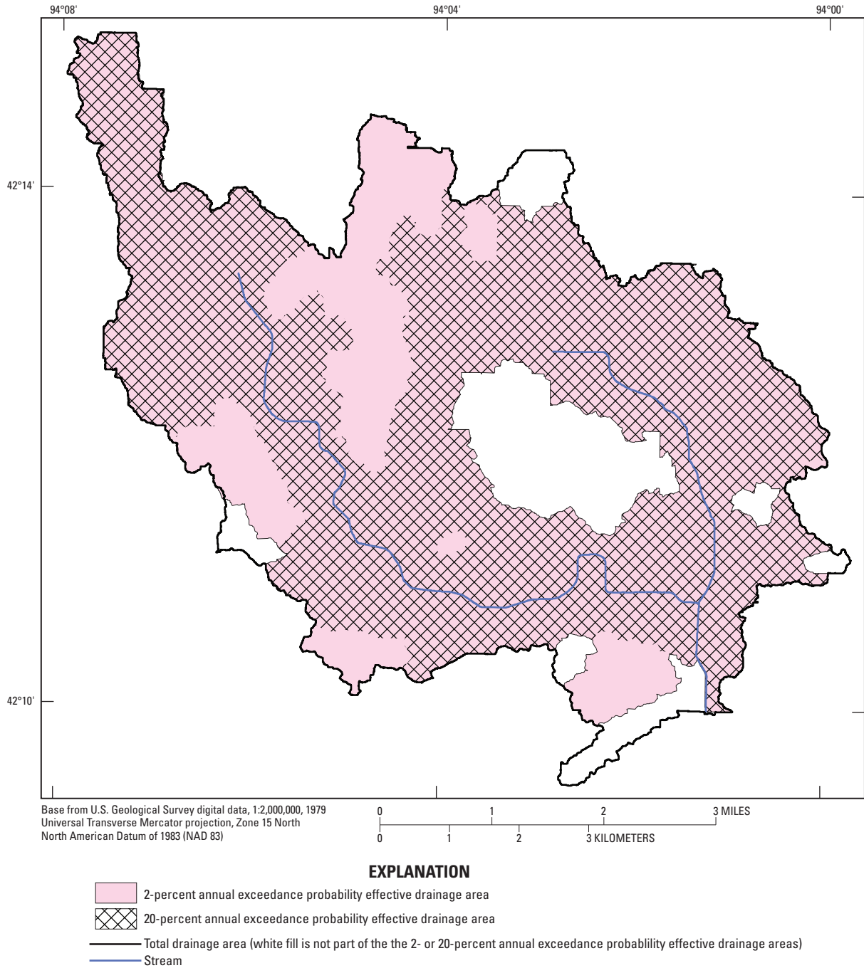
Figure 2. Example of total drainage area (23.27 square miles), 2-percent annual exceedance probability effective drainage area (20.40 square miles), and 20-percent annual exceedance probability effective drainage area (16.64 square miles) for hydrologic unit code 12 071000040703 (05481510, Bluff Creek at Pilot Mound, Iowa, site 10 in figure 1).
