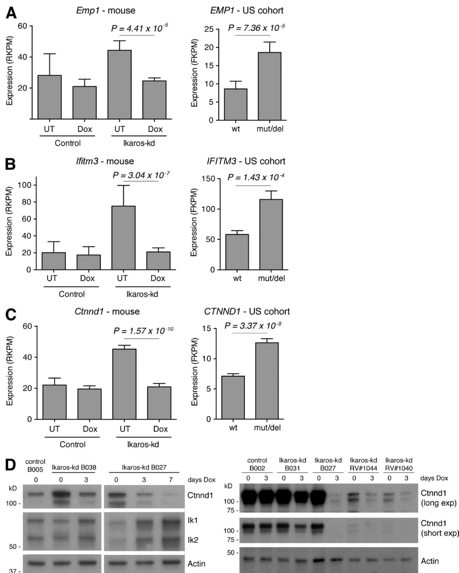
Figure 5. Regulation of IKAROS-repressed genes in mouse and human B-ALL. (A–C) RNA-seq expression (RPKM) of (A) Emp1/EMP1 , (B) Ifitm3/IFITM3 , and (C) Ctnnd1/CTNND1 in control and Ikaros-kd murine B-ALL with Dox treatments indicated (left), and the in US B-ALL cohort stratified by IKZF1 mutation status (right). P-values from moderated Student's t test. (D) Western blots of Ctnnd1 and Ikaros protein expression in multiple independent primary control and Ikaros-kd leukemias. Ikaros-kd samples B038, B027, and B031, and control samples B002 and B005 are transgenic leukemias (Fig. 1 and 2 and S1), whereas RV#1044 and #1040 were generated using the retroviral approach (Fig. S2). Actin is a loading control.
