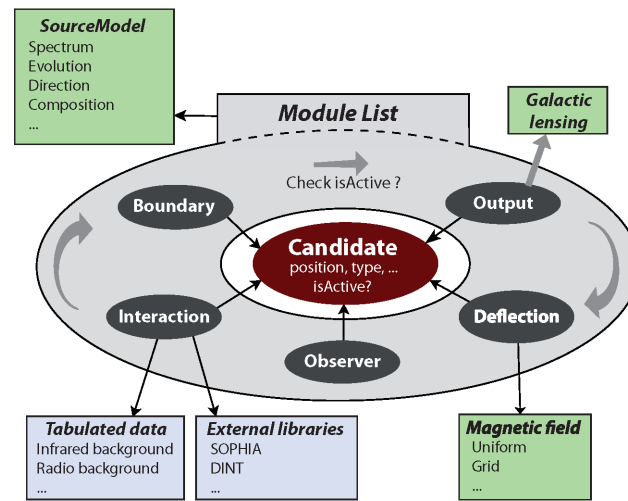
Fig. 1. Schematic overview of the modular structure of CRPropa 3, obtained from Ref. [11]. Cosmic-ray candidates are created by a source-model class. The modules only interact with this central cosmic-ray candidate, not with other modules. This continues until a certain break condition is satisfied.
