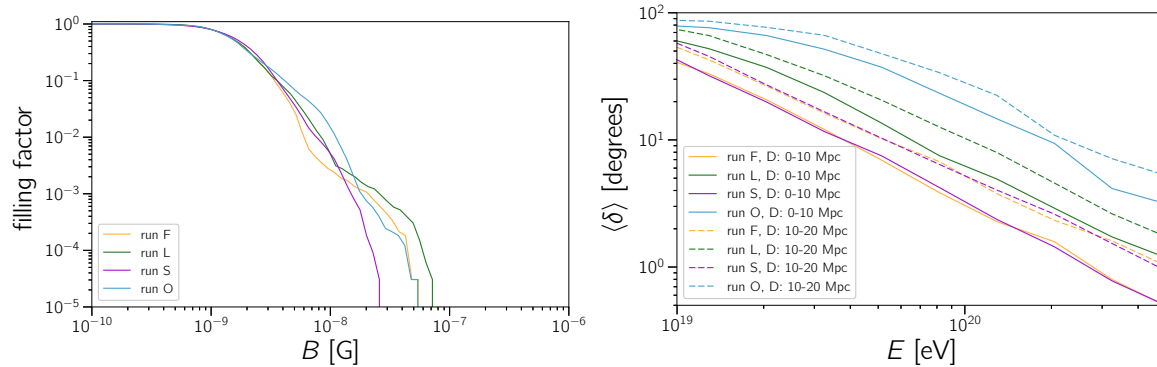
Fig. 2. The cumulative filling factors for the magnetic fields of the cosmological simulations are shown in the left panel. The average deflection of protons in the different runs are shown in the right panel for two distance bins: 0-10 Mpc (solid) and 10-20 Mpc (dashed lines). Figures adapted from Ref. [21].
