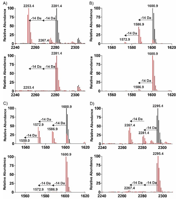
Fig. 3 Deconvoluted LC-MS data showing demethylation of methylated L-lysine (top panel) and methylated D-lysine (bottom panel) containing histone peptides in the presence of histone lysine demethylases, Fe(II), 2OG and ascorbate. A) L-H3K4me2 and D-H3K4me2 with KDM1A. B) L-H3K9me3 and D-H3K9me3 with KDM4A JmjC . C) L-H3K9me3 and D-H3K9me3 with KDM4D JmjC . D) L-H3K4me3 and D-H3K4me3 with KDM5B JmjC . (black = starting peptide, red = after KDM-catalysed reaction). Conditions for JmjC-KDM assay: 10 \mu M 2OG, 10 \mu M Fe(II), 100 \mu M Asc.
