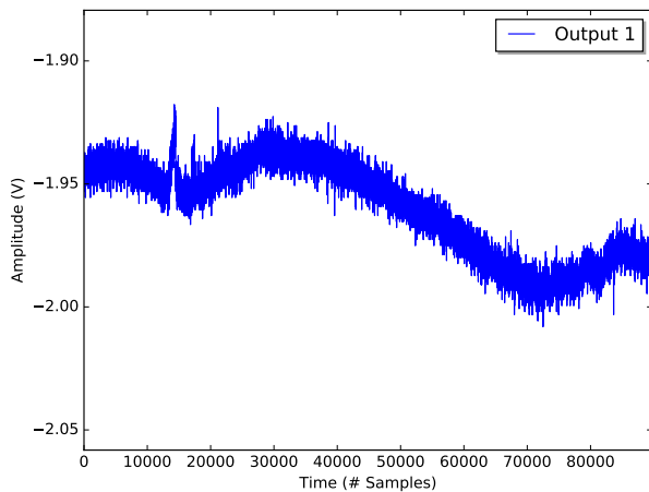
Figure 14: Aloe Vera with addition of Decanoic Acid.
