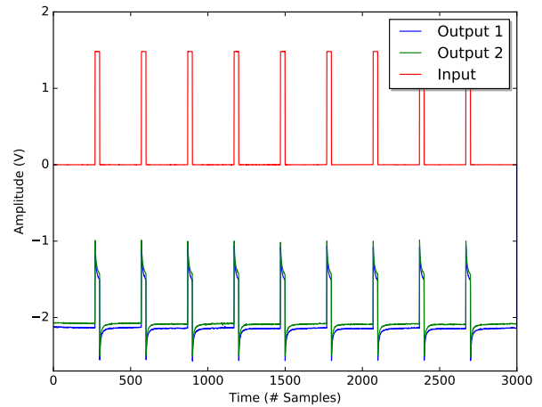
Figure 10: Echeveria action potentials in darkness.
