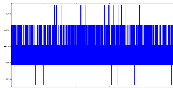
Figure 4: Control signal in Faraday cage, 1 disconnected electrode recorded for 1 second at 10kHz, peak-to-peak variation of 0.004V (negligible noise). x axis represents time and y axis represents voltage amplitude.
