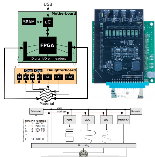
Figure 1: Mecobo setup and schematic overview.
