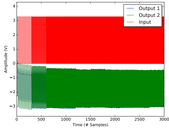
(a) Echeveria frequency sweep (1000-10000Hz) in darkness.
