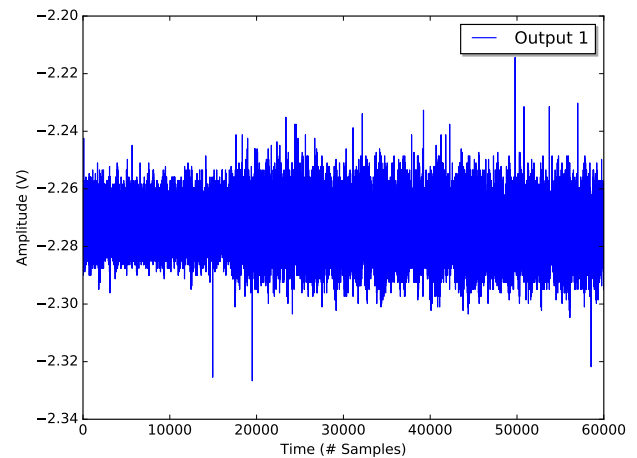
Figure 13: Echeveria with addition of NaCl salt.
