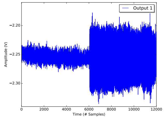
Figure 12: Aloe Vera light off 1min and on 1min.
