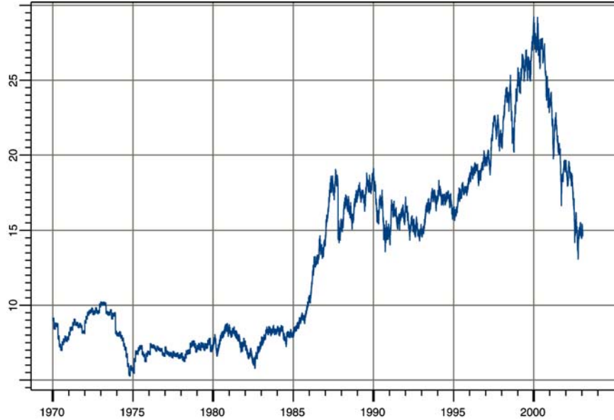
Figure 2. Normalized MSCI Y^{(\text{MSCI})}(t) for 1970–2003.
