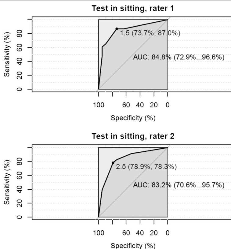
Figure 9 Receiver operating characteristic (ROC) curves. Sitting position, Rater 1 and Rater 2 with estimated area under curve AUC (95% CI). The optimal cut-off points for AUC are 1.5 and 2.5.
