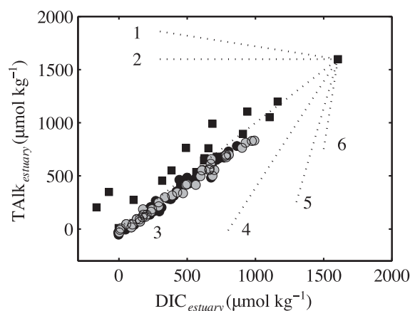
Figure 6. (a) Covariation of [\text{DIC}]_{\text{estuary}} and [\text{TALK}]_{\text{estuary}} . Black squares are samples from the Shark River during SharkTREx 1, and black and gray circles are from the Shark and Harney rivers, respectively, during SharkTREx 2. Dotted lines represent the theoretical covariation of DIC and TALK for different biogeochemical processes: (1) aerobic respiration; (2) \text{CO}_2 emission, (3) sulfate reduction, (4) \text{CaCO}_3 dissolution, (5) manganese reduction, and (6) iron reduction.
