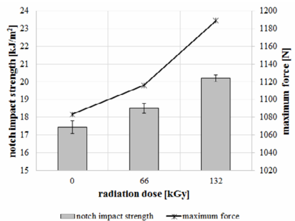
Fig. 7. Notch impact strength and maximum force (PA 7T GF 56, test temperature – 23 °C).
