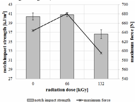
Fig. 11. Notch impact strength and maximum force (PA 7T GF 56, test temperature – 125 °C).
