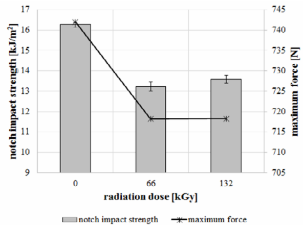
Fig. 2. Notch impact strength and maximum force (PA 66 GF 30, test temperature – 50 °C).
