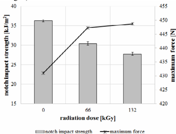
Fig. 6. Notch impact strength and maximum force (PA 66 GF 30, test temperature – 150 °C).
