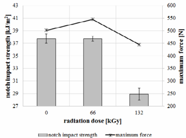
Fig. 12. Notch impact strength and maximum force (PA 7T GF 56, test temperature – 150 °C).
