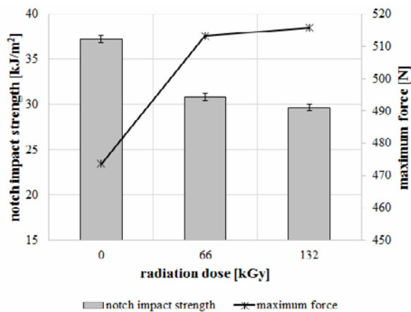
Fig. 5. Notch impact strength and maximum force (PA 66 GF 30, test temperature – 125 °C).
