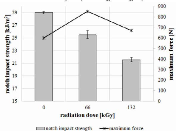
Fig. 3. Notch impact strength and maximum force (PA 66 GF 30, test temperature – 75 °C).
