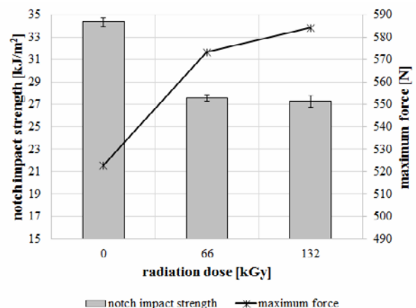
Fig. 4. Notch impact strength and maximum force (PA 66 GF 30, test temperature – 100 °C).
