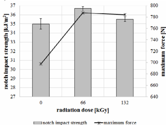
Fig. 10. Notch impact strength and maximum force (PA 7T GF 56, test temperature – 100 °C).
