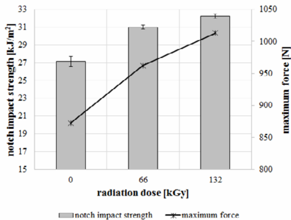
Fig. 9. Notch impact strength and maximum force (PA 7T GF 56, test temperature – 75 °C).
