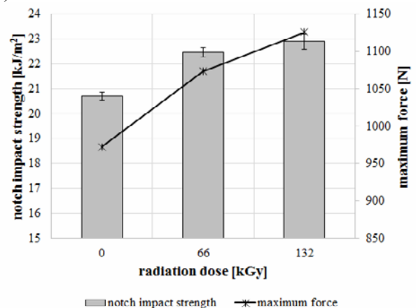
Fig. 8. Notch impact strength and maximum force (PA 7T GF 56, test temperature – 50 °C).
