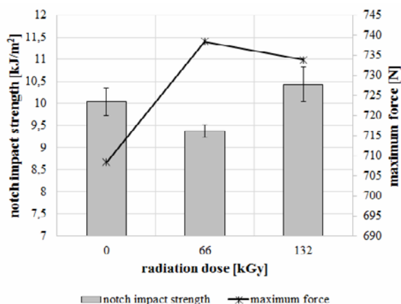
Fig. 1. Notch impact strength and maximum force (PA 66 GF 30, test temperature – 23 °C).
