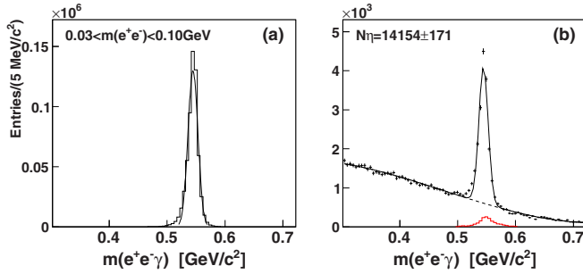
FIG. 4. m(e^+e^-\gamma) invariant-mass distributions obtained for the m(e^+e^-) range from 30 to 100 \text{MeV}/c^2 with \gamma p \rightarrow e^+e^-\gamma p candidates initially selected with the kinematic fit and allowing both e^+ and e^- to be identified with the same PID element: (a) MC simulation of \gamma p \rightarrow \eta p \rightarrow e^+e^-\gamma p fitted with a Gaussian, (b) experimental events (Run I) after subtracting the random background and the remaining background from \gamma p \rightarrow \eta p \rightarrow \gamma\gamma p . The distribution for the \eta \rightarrow \gamma\gamma background, shown by a red solid line, is normalized to the number of subtracted events. The experimental distribution is fitted with the sum of a Gaussian for the \eta \rightarrow e^+e^-\gamma peak and a polynomial of order four for the background. The total fit is depicted by a solid line, and the dashed line shows the background under the peak.
