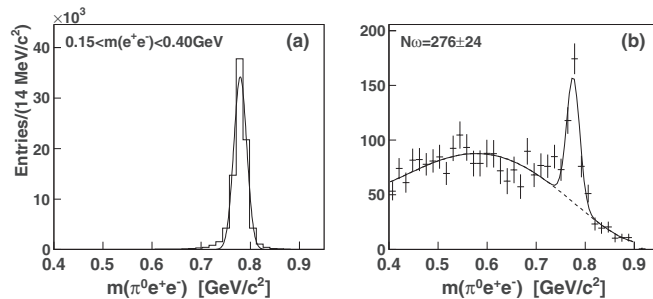
FIG. 14. Same as Fig. 11, but for the m(e^+ e^-) range from 150 to 400 MeV/ c^2 and the tighter cuts on N and R (depicted by blue solid lines in Fig. 3). The \omega \rightarrow \pi^0 \gamma background is not shown in panel (b) because it is negligibly small.
