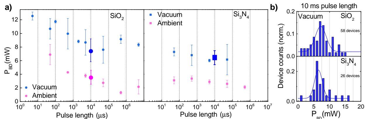
Fig. 2 a) Average breakdown power for graphene nanostructures on SiO 2 (left) and on Si 3 N 4 (right) as a function of pulse length in vacuum (blue) and under ambient conditions (pink). An average breakdown power is calculated from measurements of 2 to 5 devices (small symbols). The corresponding distribution is not shown. The error bars represent the standard deviation of these datapoints. b) Distribution of the breakdown powers for Si 3 N 4 and SiO 2 for a pulse length of 10ms in vacuum. Measurements are reported from 52 devices for SiO 2 and 24 devices for Si 3 N 4 . The lines correspond to the gaussian fit of the distribution. As a reference the mean values and the standard deviations of the fitted gaussians are represented as larger symbols panel a). Similar measurements were carried out for SiO 2 in air (large pink dot).
