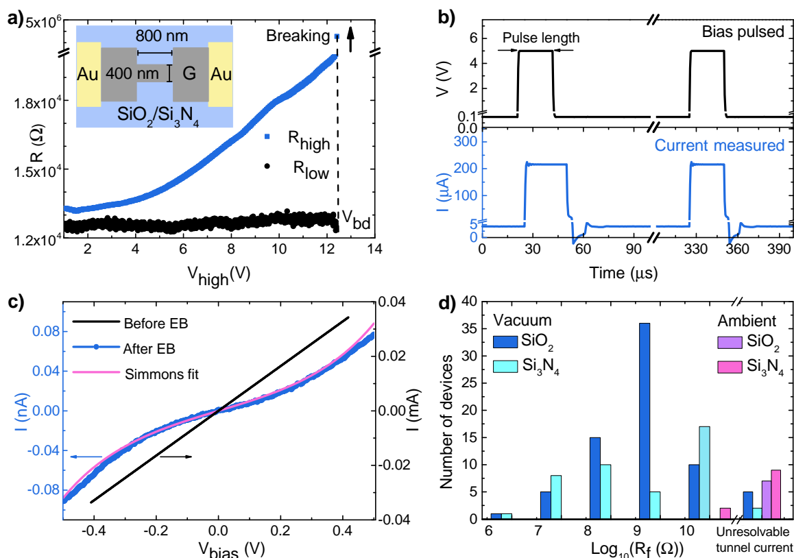
Fig. 1 Description of the EB process: a) Resistance at high bias R_{\text{high}} (in blue) and low bias R_{\text{low}} (in black) during EB of a device in vacuum with pulse lengths of 10 ms. An increase of resistance due to Joule heating is observed at high bias. At breakdown voltage V_{\text{bd}} , a jump of resistance is observed, as a sign of the gap formation. The inset is a schematic of the device. b) The applied voltage pulse is shown with the simultaneously recorded current for a pulse length of 25 \mu\text{s} . c) Current-voltage characteristic of a device before and after EB. Before EB, the I-V curve is linear and the current is in the mA range (right axis, black). After EB, we measure non linear I-V curves with currents in the nA range, due to the presence of a gap (left axis, blue). The pink curve represents a Simmons fit of the tunneling curve. d) Distribution of the low bias resistance R_f at zero gate voltage of the junctions after EB in vacuum and at ambient conditions for both substrates. For resistances larger than 10^{11} \Omega , no tunnel current could be resolved.
