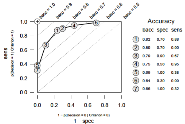
FIGURE 4: A receiver operating characteristic (ROC) curve illustrating the trade-off between sensitivity ( sens ) and specificity ( spec ) in classification algorithms. As sensitivity increases, specificity decreases (i.e., 1 - \text{spec} increases). Balanced accuracy ( bacc ) is the average of sensitivity and specificity. Ideal performance ( bacc = 1.0), is represented by the cross in the upper-left corner. The numbered circles in the plot represent the accuracy of 7 different algorithms with different trade-offs between sensitivity and specificity. Their numbers represent the rank order of algorithm performance in terms of their bacc values. (Note: The circles correspond to the fan of 7 FFTs that will be created by the ifan algorithm for the heart disease dataset in the tutorial.)
