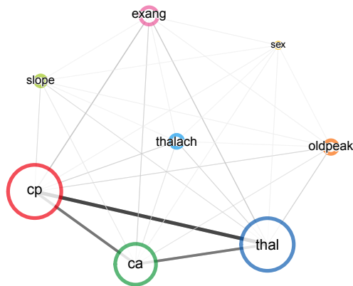
0.8 1.0 FIGURE 8: Network plot of relationships between cues in the heart disease data created by plotting an object. The object represents a bootstrap simulation of 100 FFTs trained on different random subsets of the heart disease data. The size of a node reflects how often it occurs across different FFTs in the forest (i.e., its importance), while the weight of the connection between two nodes reflects how often they co-occur within individual FFTs.
