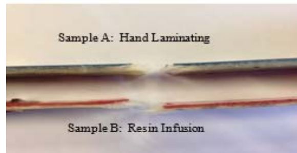
Figure-4. Fracture specimens of composite fabricated by hand lay-up method (top) and resin infusion method (bottom).
