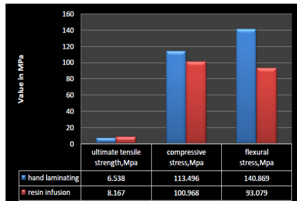
Figure-5. The comparison between three (3) types of mechanical testing for hand laminating method and resin infusion method.
