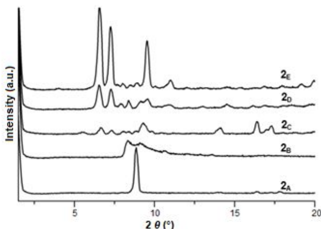
Fig 3. X-ray patterns of copper complexes 2 A-E
