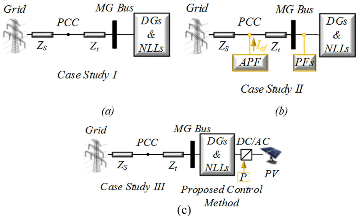
Fig 5. Schematics of a system and an MG: (a) without any compensation devices; (b) with active and passive filters; (c) using just the proposed control method on the PV.
