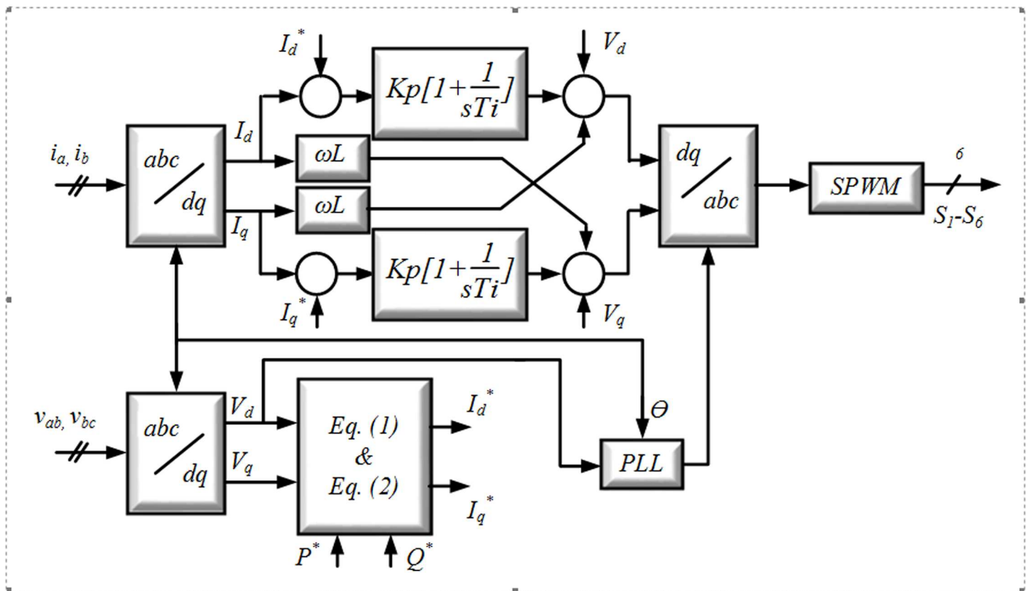
Fig 2. Block diagram of the control active and reactive powers.
