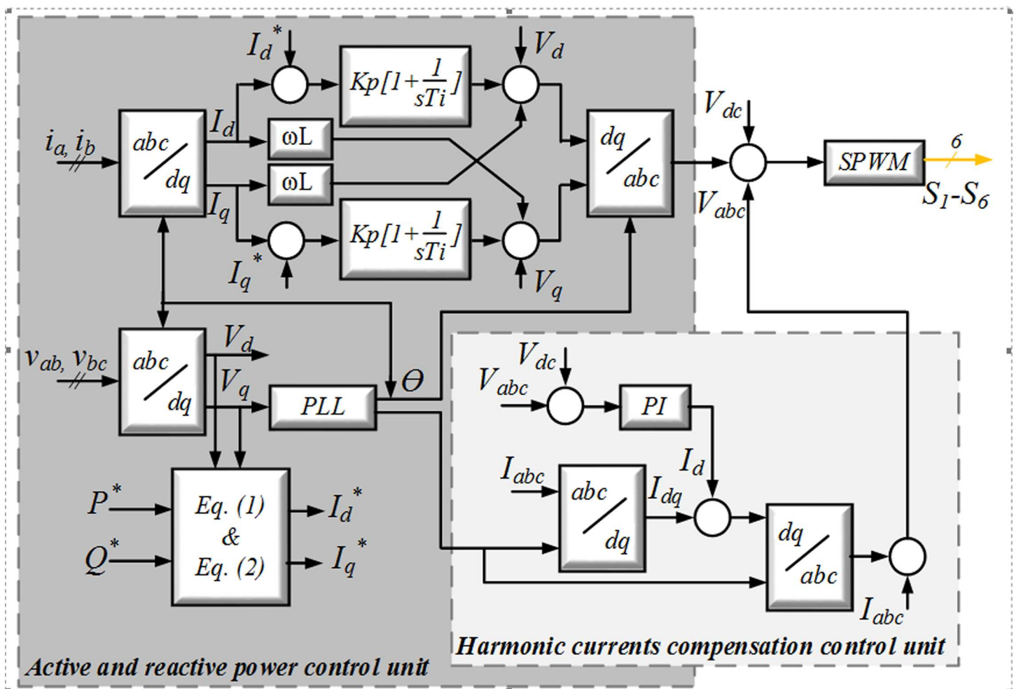
Fig 1. Block diagram of the GCI's proposed control method.
