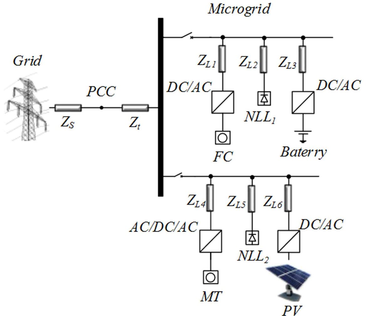
Fig 4. Study system configuration with DGs and distorted loads.
