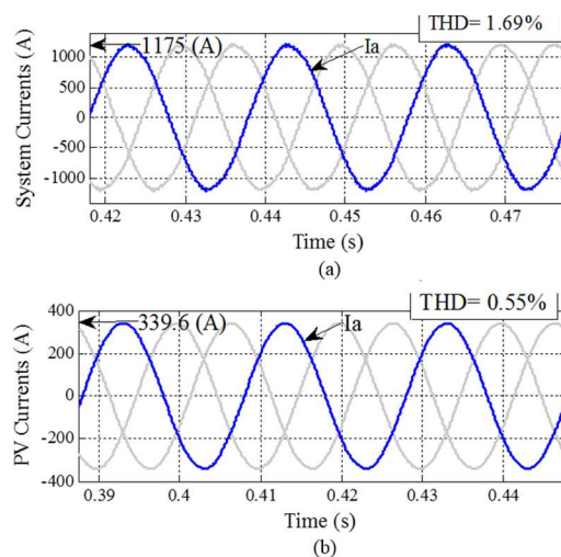
Fig 10. System and DG unit current waveforms with THD without any compensation devices except for the proposed control method on the PV: (a) system currents; (b) PV currents.
