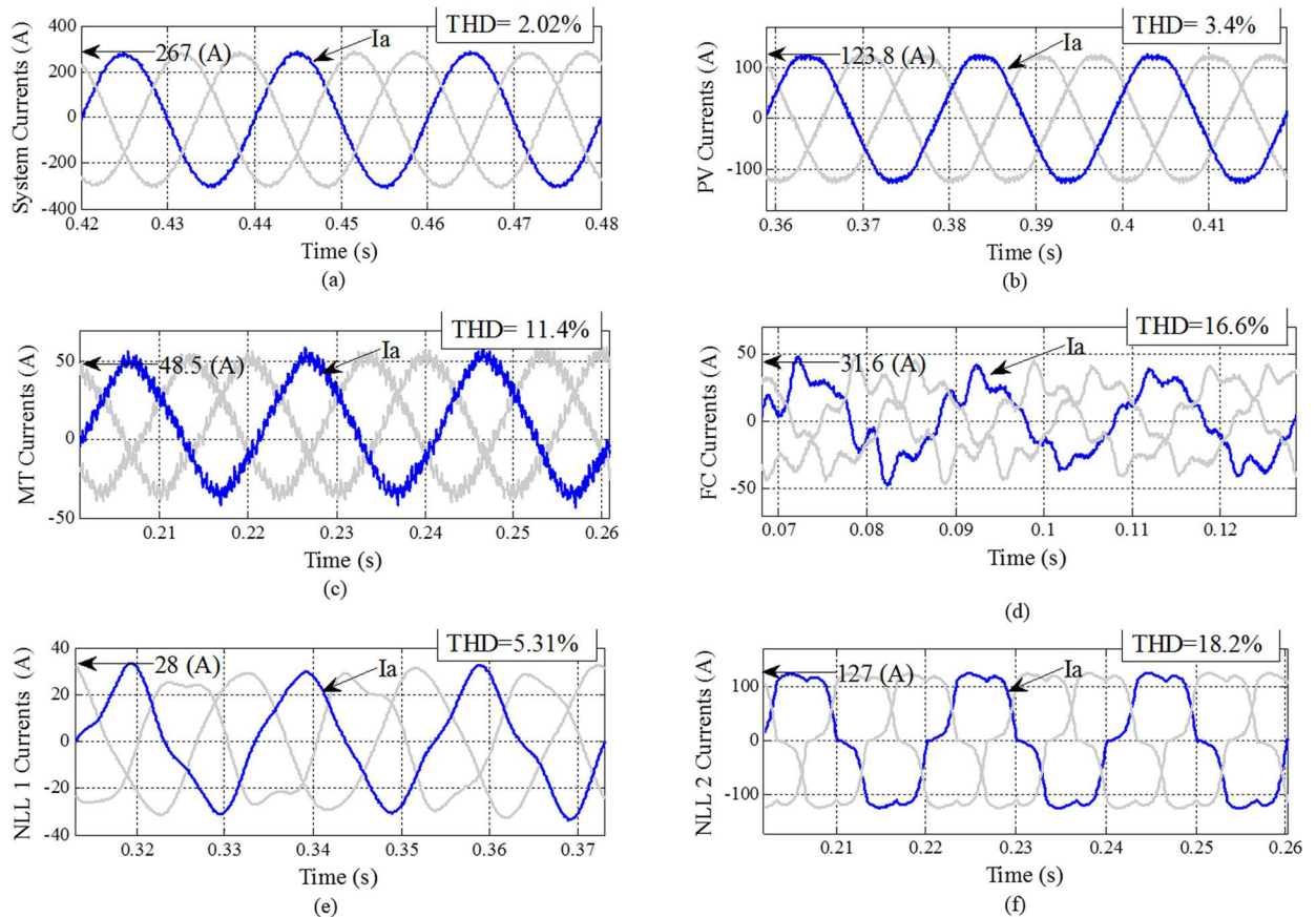
Fig 8. System DG unit current waveforms with THD after compensation with active and passive filters: (a) system currents; (b) PV currents, (c) MT currents; (d) FC currents; (e) NLL 1 currents; (f) NLL 2 currents.
