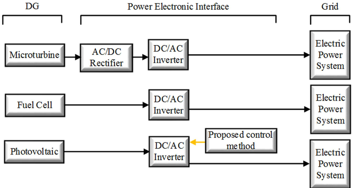
Fig 9. Block diagram of the power electronic interface configuration.
