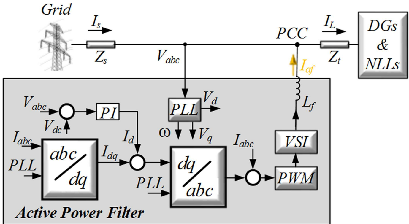
Fig 7. Block diagram of the control system for the APF.
