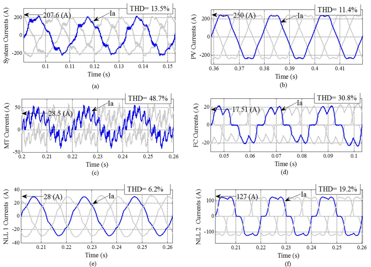
Fig 6. System DG unit currents and NLL current waveforms with THD without any compensation: (a) system currents; (b) PV currents; (c) MT currents; (d) FC currents; (e) NLL 1 currents; (f) NLL 2 currents.
