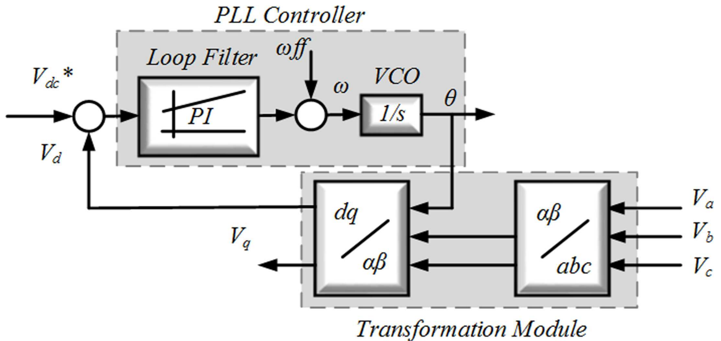
Fig 3. PLL structure of the three phase.
