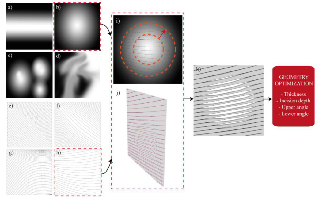
Fig. 3. Geometry generation steps (a, b, c, d) Random bitmap image to control opening position and incision depth; (e, f, g, h) Random field line pattern; (i, j) Color gradient variation that influence the openings dimensions; (k) Final shading system geometry.
