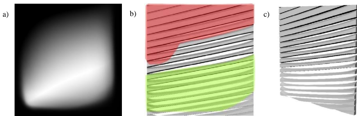
Fig. 7. (a) Bitmap image defines openings position and incision depth; (b) Front view of proposed concrete shading panel. The proposed solid zone to avoid glare is marked in Red. The proposed outdoor vision zone is marked in green; (c) Perspective view of shading system.
