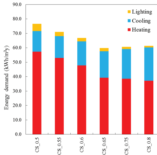
Fig. 5. Energy demand results with different shading systems configuration, depending on d/D ratio.
