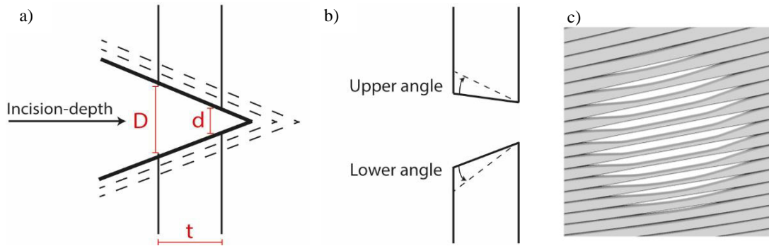
Fig. 4. Main variation parameters in geometry definition (a) Incision depth, d/D factor; (b) Upper and lower angle rotation (from 0^\circ to 25^\circ ); (c) Concrete shading system selected for simulation phase.
