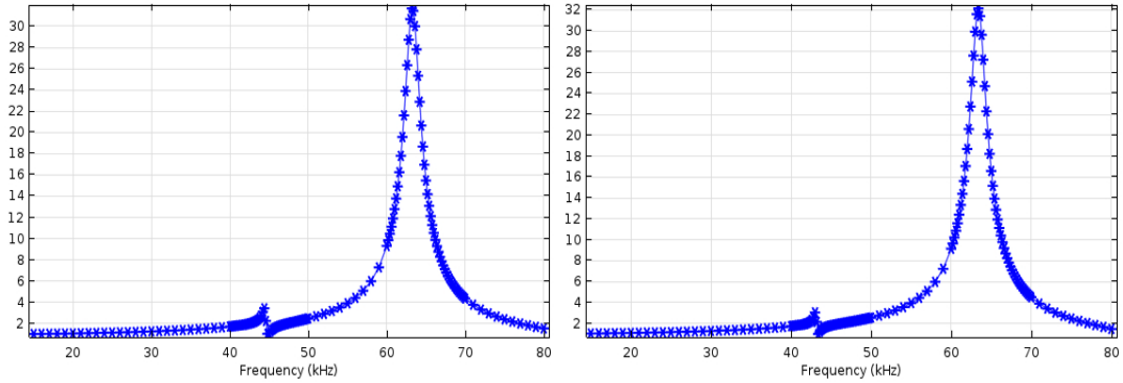
Figure 6: Vertical displacement spectra [ \mu\text{m} ] for the center point of the membrane belonging to the axis of symmetry by COMSOL Multiphysics 5.2: t_{cap} = 80 \mu\text{m} , R_{hole} = R_{PMUT}/3 , H_{cap} = 200 \mu\text{m} (left), 500 \mu\text{m} (right).
