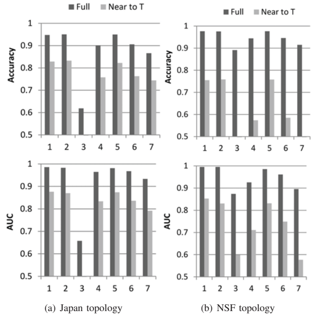
Fig. 5: Accuracy and AUC depending on the feature set selection, for datasets A (left) and B (right)
