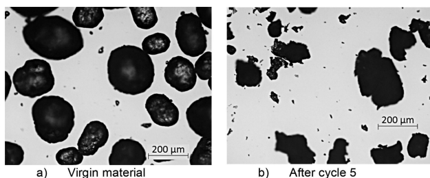
Figure 3. Raw-AN particles viewed under microscope (magnification: 5 ×)
