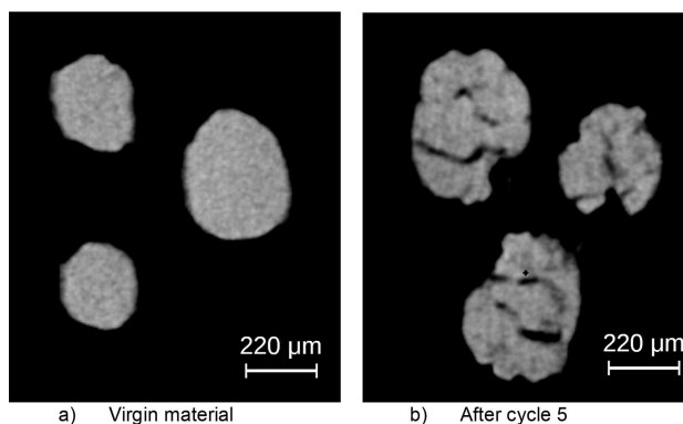
Figure 5. Tomographic slices of Raw-AN particles before and after five thermal cycles (Pixel pitch = 5.5 μm/pixel)
