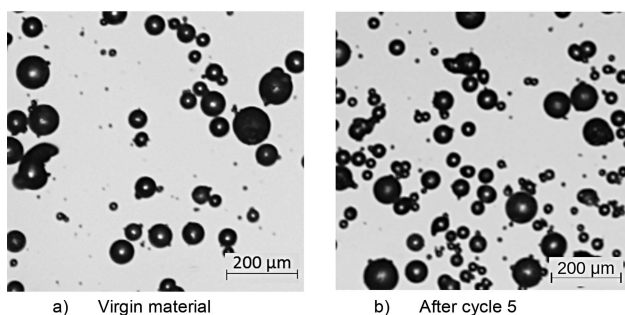
Figure 4. PSAN-Coarse particles viewed under microscope (magnification: 5 ×)
