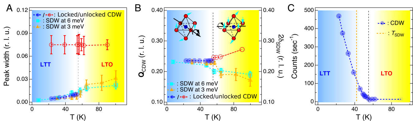
Fig. 3. Decoupling of the CDW and SDW in the high-temperature phase. (A–C) The results of fitting the quasi-elastic intensity showing (A) the full width at half maximum, (B) the incommensurability, and (C) the intensity at the peak. The black dashed line at 54 K corresponds to the LTT–LTO (low-temperature orthorhombic) structural phase transition which is depicted in B , and blue and yellow code temperatures below and above this threshold (29). The orange dashed line at 42 K in C represents the static SDW transition. The behavior of the SDW, taken from inelastic neutron scattering results at 3 and 6 meV energy transfer from ref. 10, are included on A and B . We see that the CDW and SDW incommensurabilities evolve in different directions above 54 K, which indicates a decoupling of the charge and spin degrees of freedom. We also note that the high-temperature CDW width and intensity show no detectable changes through the LTT–LTO transition (any possible changes would be smaller than our error bars, which are obtained from the least-squares fitting algorithm).
