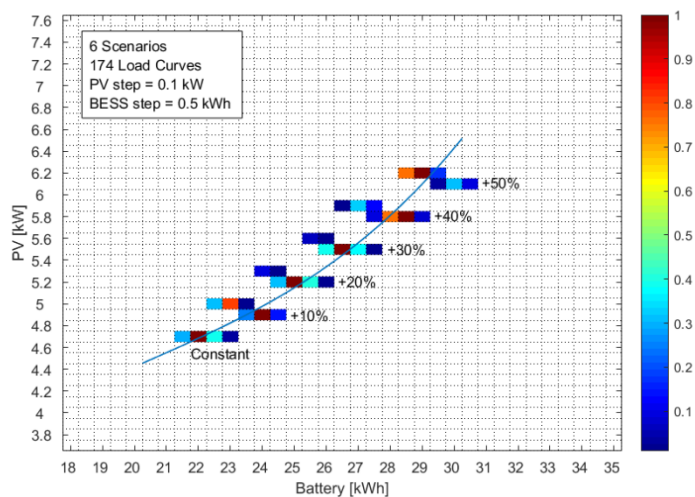
Fig. 8. PV+BESS micro-grid robust design: map of solutions (the rainbow colormap helps in normalizing the frequency of occurrence of each PV-BESS combination with respect to the most frequent optimum plant in each scenario).
