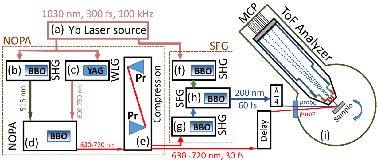
Fig. 1. Schematic drawing of the in house - developed system to measure trCD-ARPES. (a) Yb:KGW laser source (b) second harmonic generation (SHG) doubling the laser fundamental frequency, (c) white light supercontinuum (WLC) generated inside a YAG crystal. (d) WLC seed pumped 515 nm beam focused inside a 2 mm BBO crystal generating the ultrabroadband NOPA signal. (e) NOPA dispersed by a pair prism (Pr) compressor. The output compressed NOPA is then split. One portion goes to a motorized delay stage and is directly used as ultrashort tunable pump. The other fraction is frequency doubled in (f) to generate the ultraviolet probe. In (g), the 515 nm beam (e) and the SHG 335 nm beam (f) generate the 203 nm probe beam in a sum frequency generation (SFG) process. The probe goes through quarter-wave plate and is focused on the sample (h) shows the ultrahigh vacuum photoemission chamber, equipped with a time of flight (ToF) analyzer. The ToF records the flight-time of the photoelectrons collected by micro channel plate (MCP) detector.
