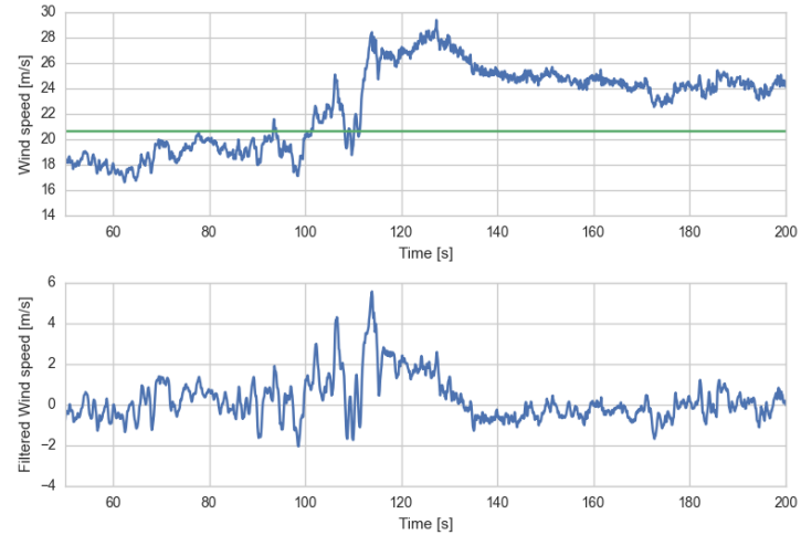
Fig. (2) Above: The measured wind speed at 100 m height (blue) and the 30 s-mean wind speed preceding the peak (green). Below: The corresponding filtered wind speed signal, including the effect of rotational sampling.
