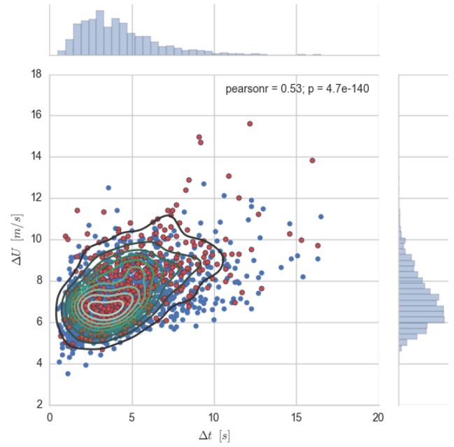
Fig. (4) The joint distribution of rise times and velocity jumps of the detected gusts.
