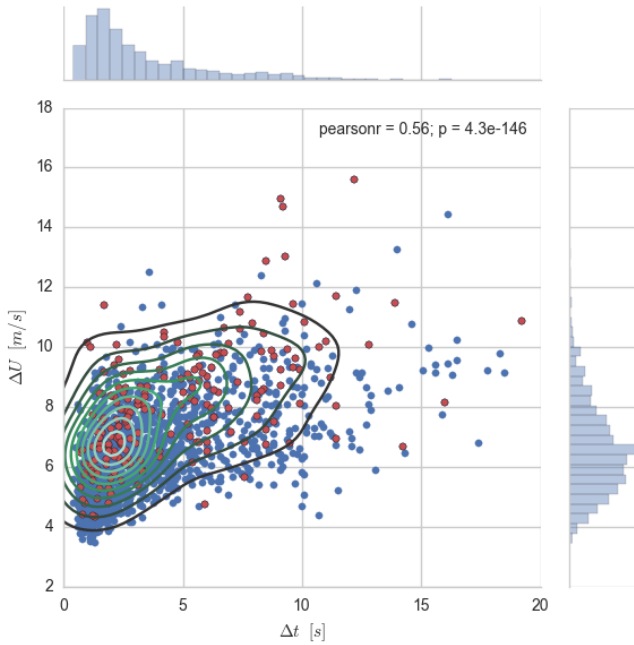
Fig. (3) The joint distribution of rise times and velocity jumps of the detected gusts.
