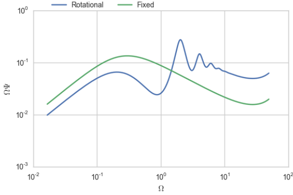
Fig. (1) The normalized rotationally sampled power spectrum (blue) and the fixed point von Kármán spectrum (green).
