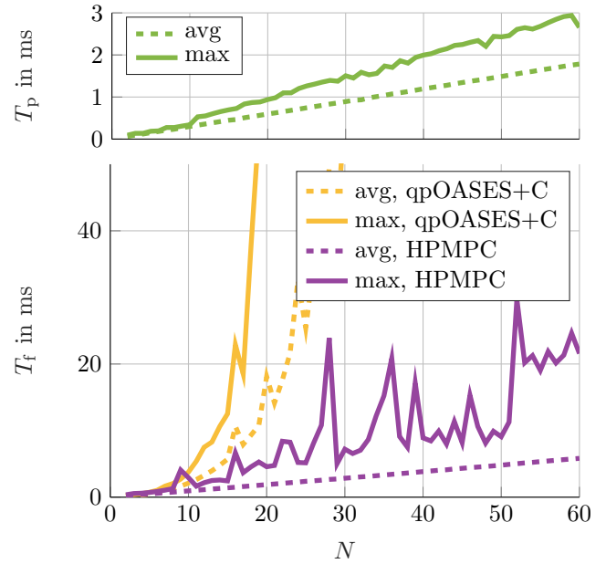
Fig. 4. CPU time of preparation phase T_p and feedback phase T_f depending on horizon length N .
