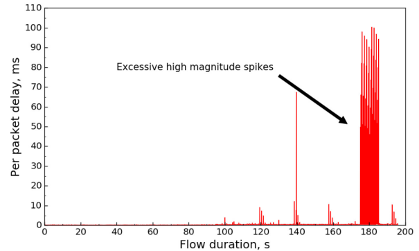
Figure 13: Per-packet delay of a migrated flow (15-30-45 pps set)
