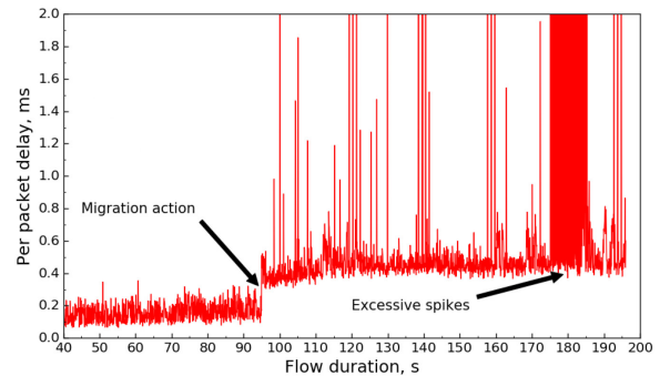
Figure 14: Per-packet delay of a migrated flow (a fragment of Figure 13)
