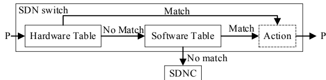
Figure 2: Proposed pipeline processing
