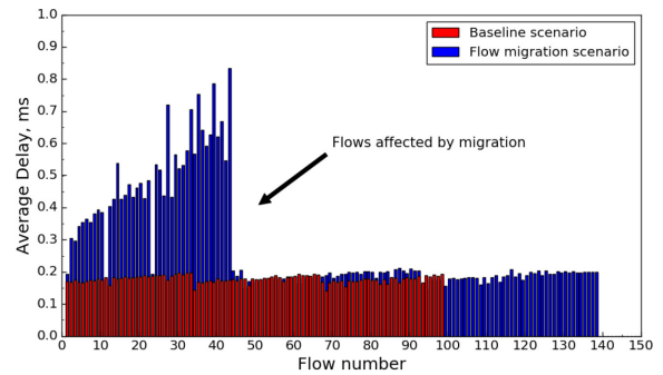
Figure 8: Baseline vs Flow migration scenario. Rate group set: 10-20-30 pps
