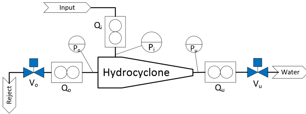
Figure 2: P&ID of the hydrocyclone at the pilot plant.
