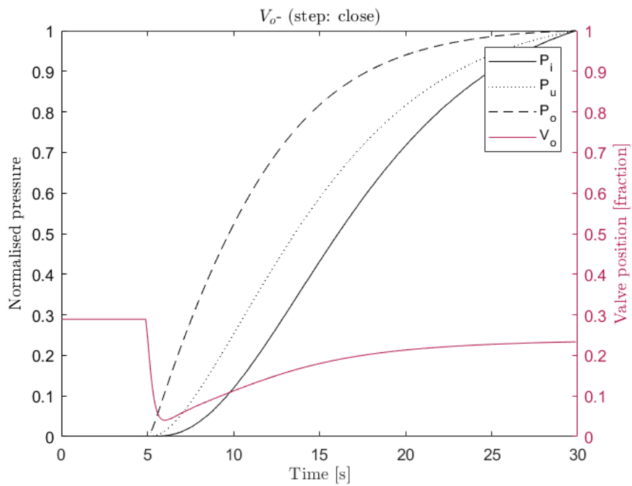
Figure 7: Response to closing overflow valve V_o in DPS.
