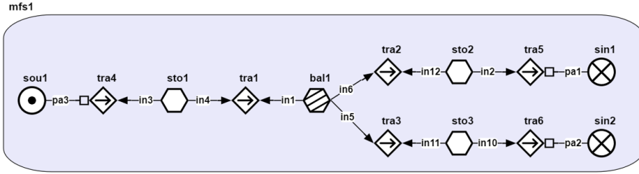
Figure 3: MFM Model of hydrocyclone mass flow separation.
