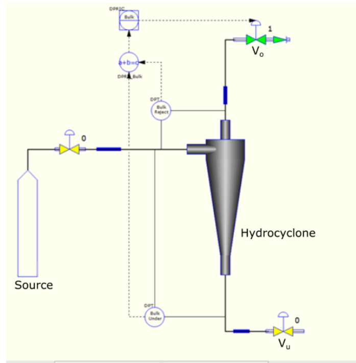
Figure 6: Model of the hydrocyclone in K-Spice.
