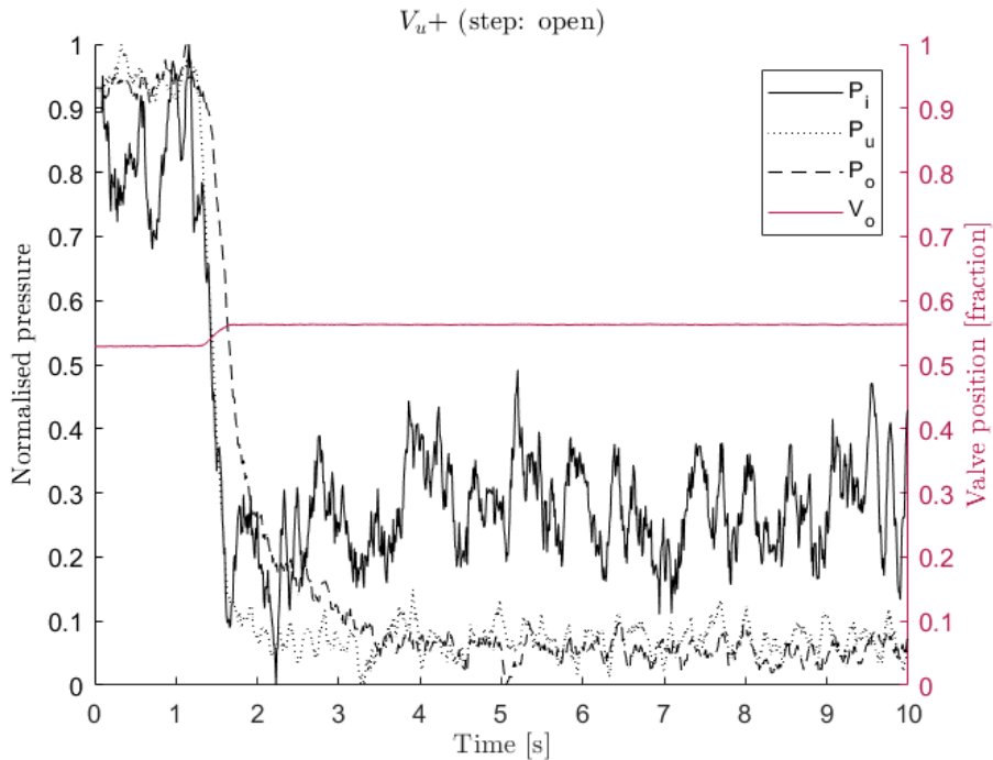
Figure 8: Response to opening underflow valve V_u on the Pilot Plant.
