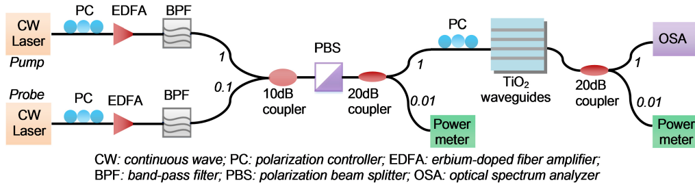
Fig. 5. Experimental setup for performing FWM experiments in the fabricated TiO 2 waveguides.
