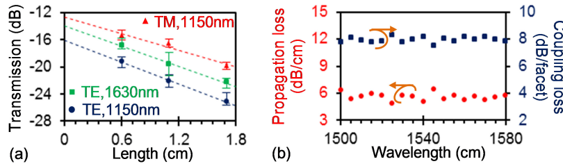
Fig. 3. (a) Transmission as a function of the waveguide length for the fabricated TiO 2 waveguides with different widths and for different polarizations at wavelength 1550 nm. Linear fittings are given as dashed lines. (b) The propagation loss (red circles) and coupling loss (blue squares) at different wavelengths in the waveguide with w_1 = 1150 nm for the TE mode.
