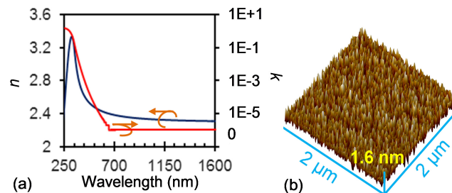
Fig. 1. (a) The measured index ( n ) and extinction coefficient ( k ), and (b) an AFM image of the deposited \text{TiO}_2 film.
