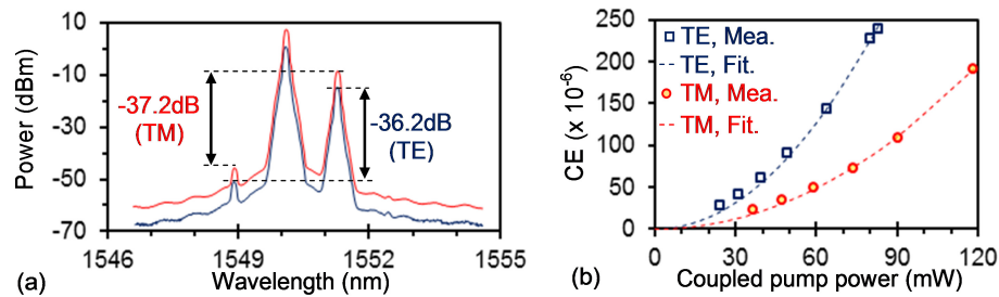
Fig. 6. FWM spectra for the TE- (blue) and TM- (red) modes in a waveguide with w_1 = 1150 nm and L = 1.1 cm for the maximum input pump powers. (b) The conversion efficiency (CE) with respect to different coupled pump powers for both the TE- (blue) and TM- (red) modes.
