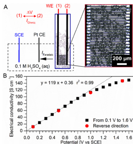
Figure 5. (A) Schematic diagram of electrochemical apparatus for in situ conductance studies in 0.10 M H 2 SO 4 . cNPGFs were uniformly deposited on interdigitated electrodes. Ohmic current was probed by keeping fixed bias between electrodes (1) and (2), during application of increasing and decreasing constant potential in the three-electrode system (saturated calomel electrode (SCE) as reference electrode (RE), Pt counter electrode (CE) and as working electrode (WE), respectively). (B) Apparent electrical conductivity vs applied potential for a typical cNPGF, together with the fitting line and corresponding equation.
