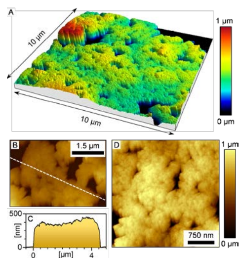
Figure 3. AFM images of cNPGF. (A) Large area ( 10 \times 10 \mu\text{m}^2 ) 3D image showing micro scale uniform film. (B-C) Height analysis of AFM image, showing a thickness of around 400 nm. The height profile in (C) is taken along the dashed line in (B) and indicates a place of cross-section plot (C). (D) High magnification of cNPGF.
