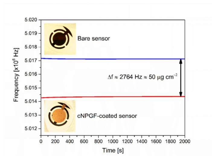
Figure S1. Typical massograms obtained during recording of QCM signals of bare (blue line) and cNPGF-coated (red line) sensors in air. The difference in frequency of oscillating sensors yields apparent areal density of deposited film.
