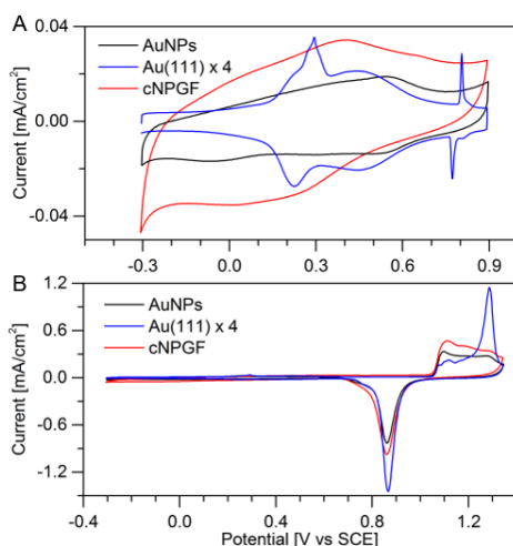
Figure 4. Cyclic voltammograms of Au(111), AuNPs and cNPGF in (A) narrow and (B) broad potential window. Cyclic voltammograms were recorded at 50 mV/s in 0.10 M \text{H}_2\text{SO}_4 . The current densities related to Au(111) were increased four-fold for better comparison.
