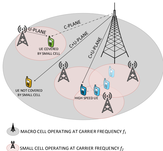
Fig. 2. HetNet with C/U plane split architecture. High-speed UEs and those not covered by the small cells receive data and control from the macro cell. UEs covered by the small cells receive control from the macro cells and data from the small cells.
