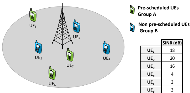
Fig. 6. Single cell scenario for user pairing example in NOMA.
