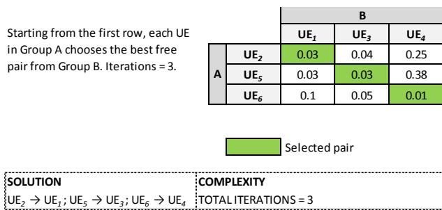
Fig. 9. Random pairing application on a user pairing example for NOMA.
