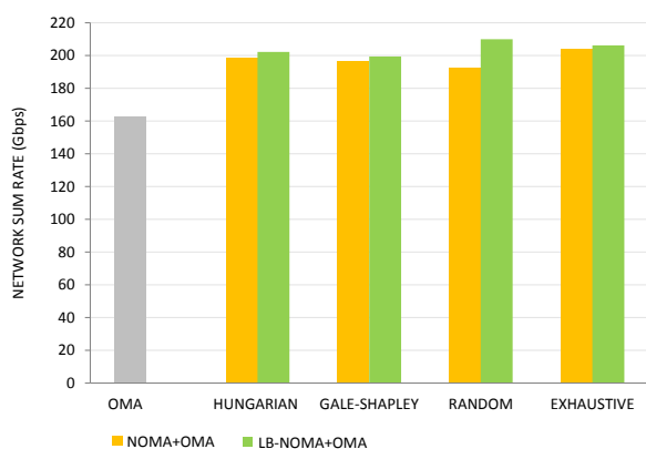
Fig. 14 Network sum rate comparison for the modeled HetNet.
