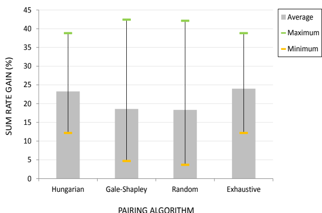
Fig. 11. Sum rate gain for a single cell for four pairing algorithms for NOMA; OMA is used as the benchmark.
