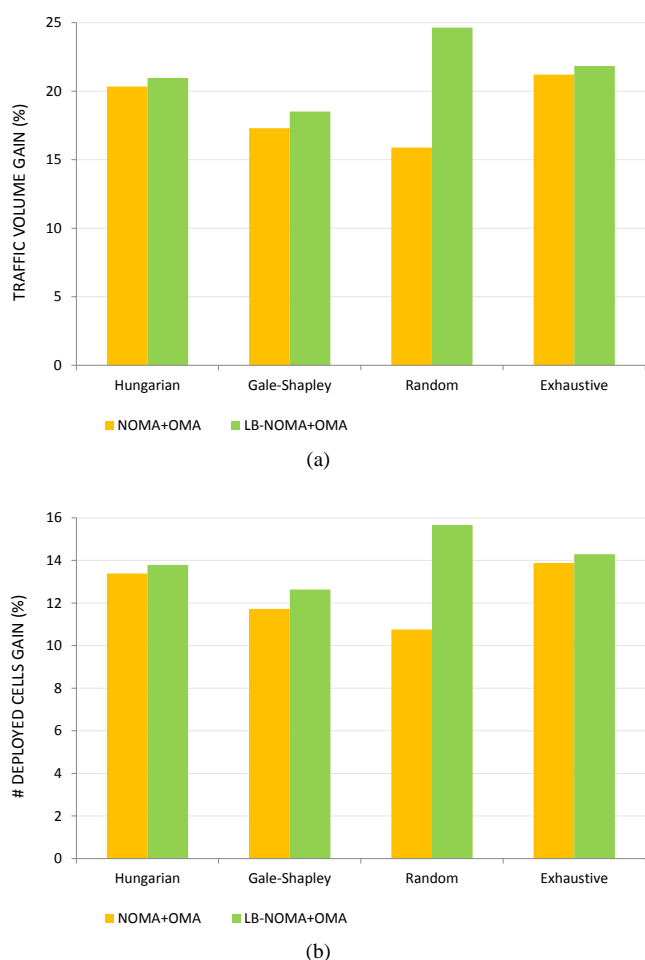
Fig. 17 Gain for the modeled HetNet for four pairing algorithms for NOMA; OMA is used as the benchmark: a) Traffic volume gain; b) Number of deployed cells gain.
