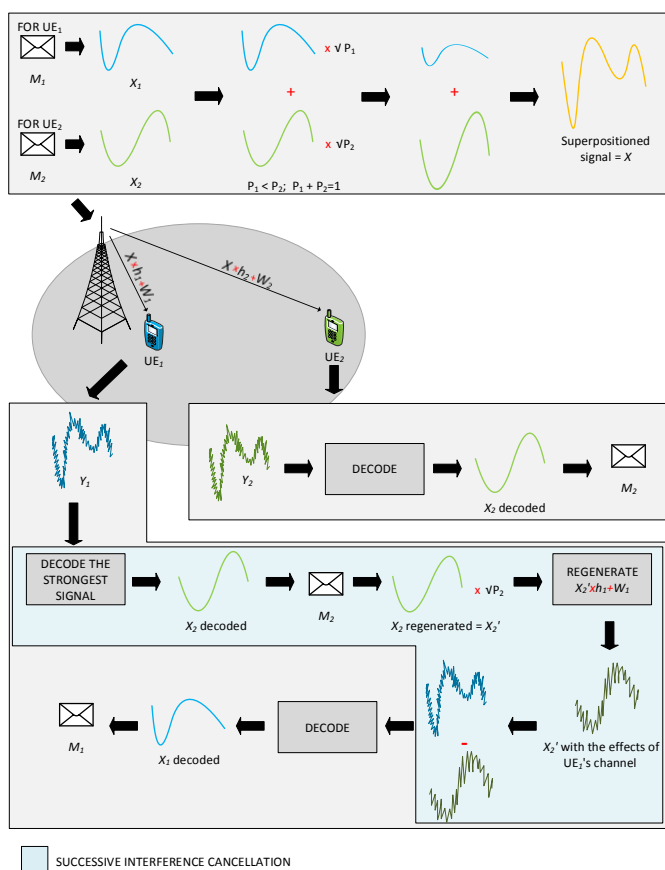
Fig. 5. Transmission and reception of signals in NOMA for two users.
