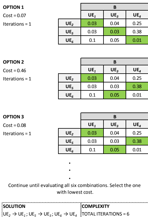
Fig. 10 Exhaustive pairing application on a user pairing example for NOMA.
