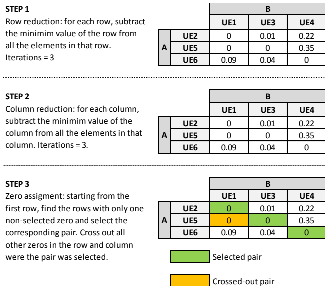
Fig. 7. Hungarian method application on a user pairing example for NOMA.
