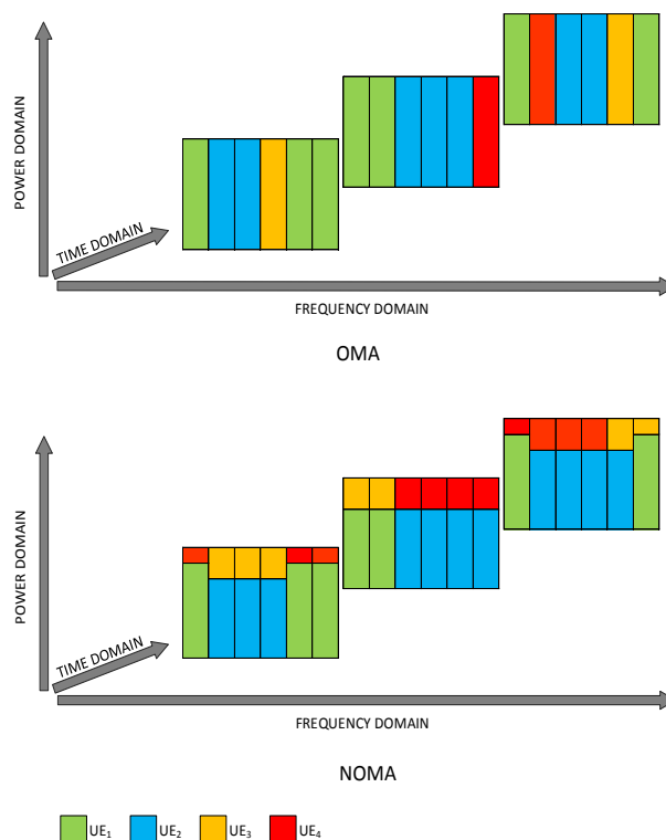
Fig. 3. Users multiplexing differences between OMA and NOMA.
