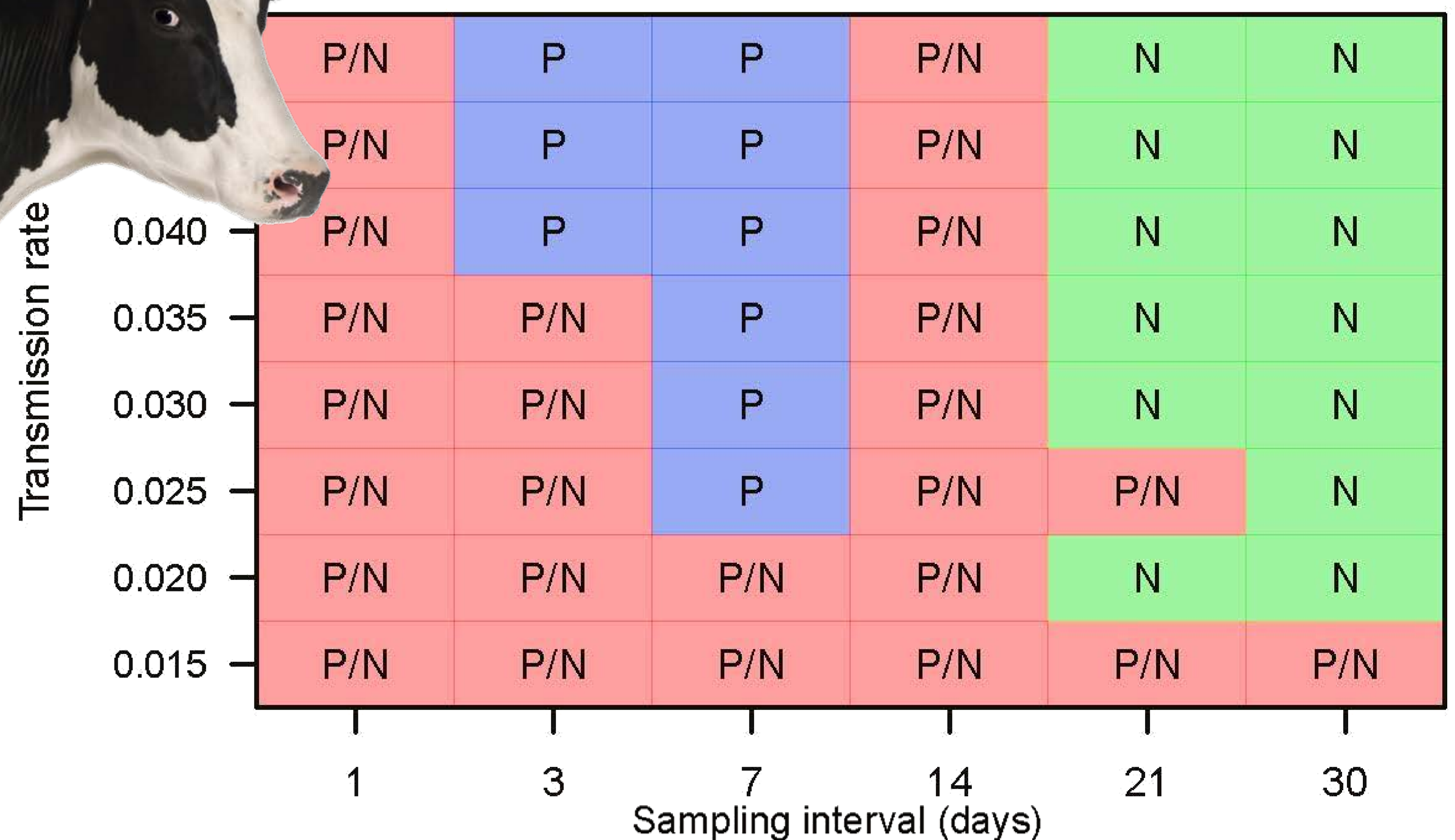
Figure 1: The optimal method for the true transmission rate and sampling interval. Letters show whether Poisson regression (P) or the New method (N) performed significantly better than or equally good as Poisson regression (P/N).
