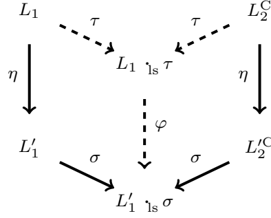
Fig. 4 The substitutions of the lifting lemma. An arrow from L to L' labeled with \eta indicates that L \text{is} \eta = L' . Full arrows are relations we know. The dashed ones are established in the proof of the lemma by noticing that \eta \cdot \sigma is a unifier of L_1 and L_2^C , which means we can obtain the MGU \tau and by the definition of MGUs also \varphi .
