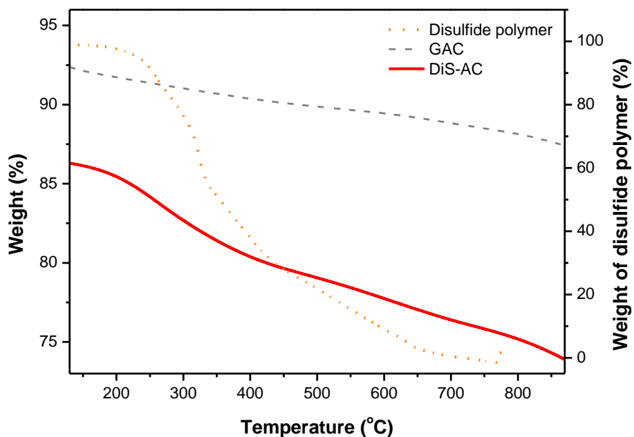
Figure 4.5 Thermo-gravimetric analysis of bare GAC (dashed line), the pure disulfide polymer (dotted line) and the grafted polymer DiS-AC (solid line) (Paper III).
