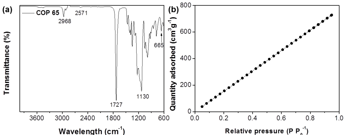
Figure 2.6 (a) IR spectrum of COP-65. The strong peaks in the 1130–1727 \text{cm}^{-1} region correspond to the C-O and C=O bonds. The small peak at 665 \text{cm}^{-1} shows the C-S bonds. (b) The \text{N}_2 adsorption isotherm measured at 77 K.
