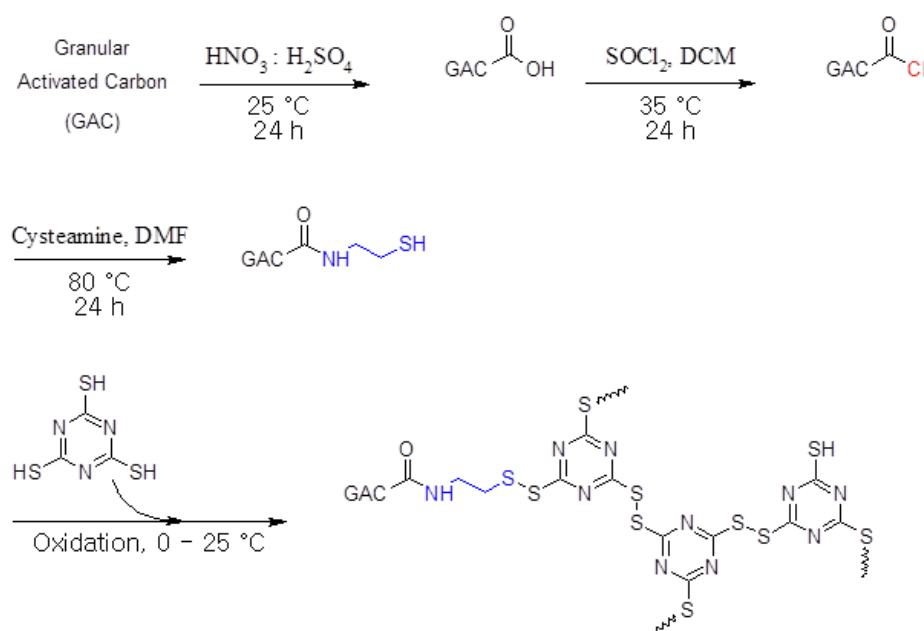
Figure 4.2 Step-wise procedures for DiS-AC formulation. Initially, bare GAC oxidized and modified through acyl chlorination. Afterwards, cysteamine attachment conducted on the surface modified GAC. Finally, the polymer grafting has been implied on the cysteamine attached GAC (Paper III).
