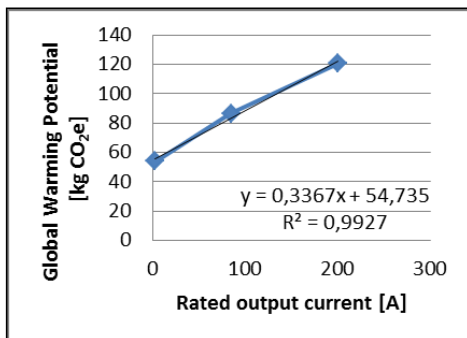
Figure 10: GWP for APCBs of 3 A, 85 A and 200 A with respect to the nominal output current with the derived linear approximation
