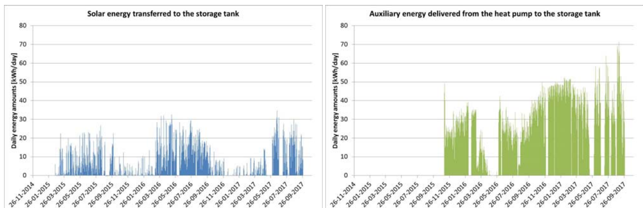
Figure 30. Daily energy amounts charged to the storage tank in the test period.
