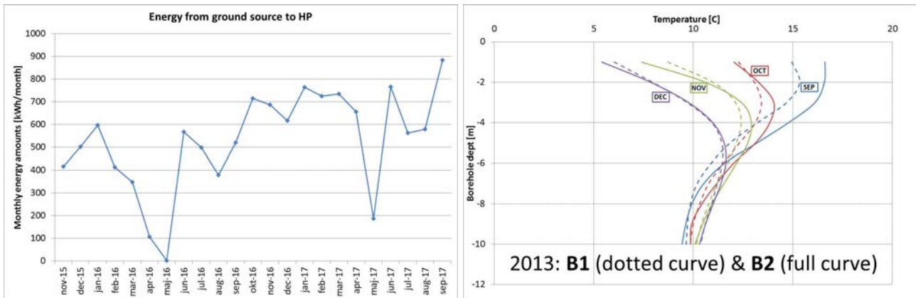
Figure 67. Left: Monthly amount of energy drawn from the ground source, November 2015 – September 2017. Right: Ground temperatures from the middle of each month in 2013.
