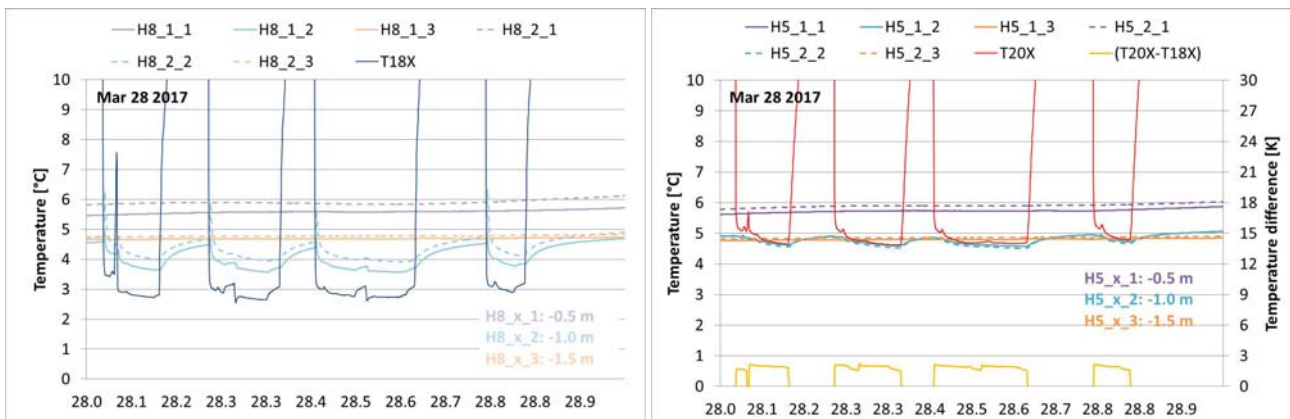
Figure 21. Temperatures in the ground above, next to and below the hoses in the inner sling on March 28 2017. H_8_1_z and H_8_2_z show the temperatures at the sling inlet and H_5_2_z and H_5_1_z show the temperatures at the sling outlet.
