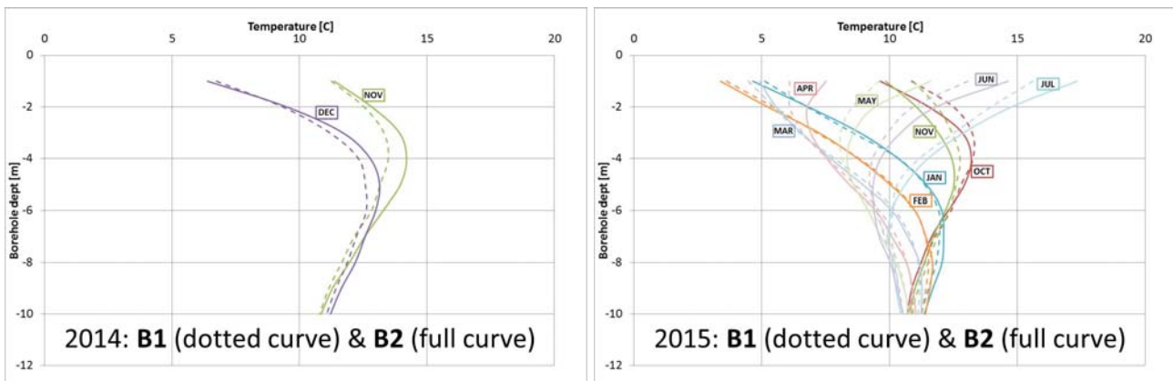
Figure 68. Ground temperatures from the middle of each month in 2014 and 2015.
