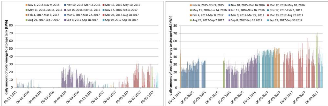
Figure 52. Daily energy amounts charged to the storage tank in the test period with good measurements.
