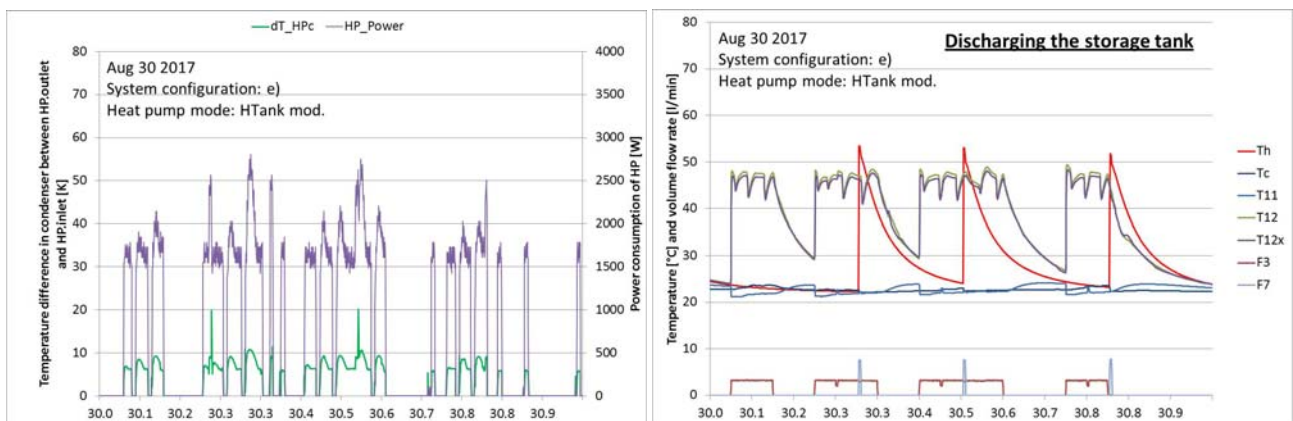
Figure 23. Power consumption of heat pump compressor, temperatures and flows in the system on August 30 2017.
