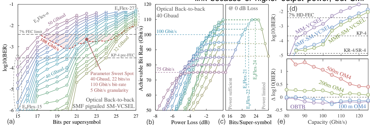
Fig. 2: (a) BER performance vs. the number of bits per super-symbol for different symbol rate values; (b,c) Achievable bit rate for different numbers of bits per super-symbol; (d) BER performance for different types of VCSEL modules in OBTB mode; (e) BER difference between MMF- and SMF-pigtailed SM-VCSELs vs. channel capacity for different MMF links at 40 Gbaud symbol rate.
