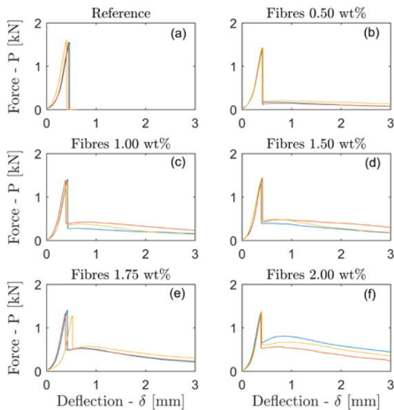
Fig. 6. Load-deflection curves for gypsum prisms. (a) control specimen, (b) fibre content 0.5 wt%, (c) fibre content 1.0 wt%, (d) fibre content 1.5 wt%, (e) fibre content 1.75 wt%, (f) fibre content 2.0 wt%
