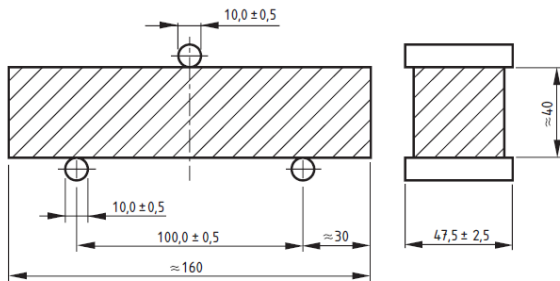
Fig. 4. Setup for three-point bending test (DS/EN-196-1-1, 2005)
