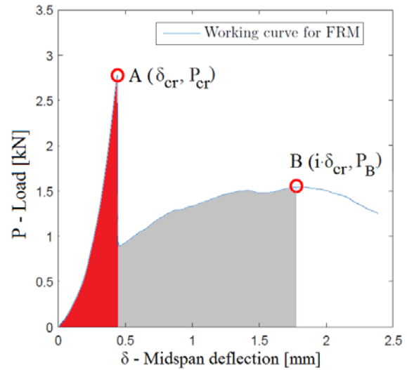
Fig. 5. Theoretical working curve for a fibre reinforced material (FRM) from a three-point bending test
