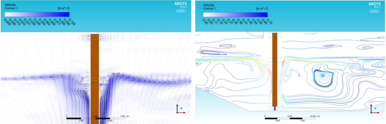
(A) Velocity vectors showing the uprising flow (B) Stream lines shown a big circulation
