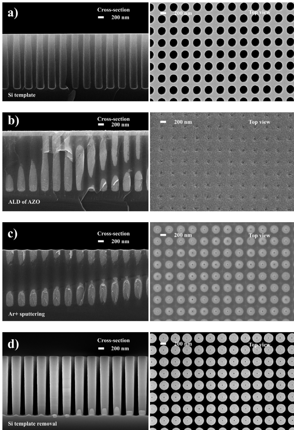
Figure 6.10: SEM verification for each fabrication step of pillars production. Left side shows cross-sectional images and right side of the Figure shows the top view of the structures. Each step a)-d) are in the same order as presented in Figure 6.9
