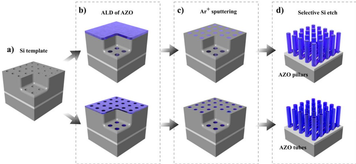
Figure 6.9: Schematic drawing of the pillars and tubes fabrication: a) SOI template with DRIE etched holes, b) ALD deposition of AZO D25 250 \text{ }^\circ\text{C} . Complete filling for HMM pillars or partial for tubes. c) The top layer removal. d) Selective Si etch using conventional RIE process.
