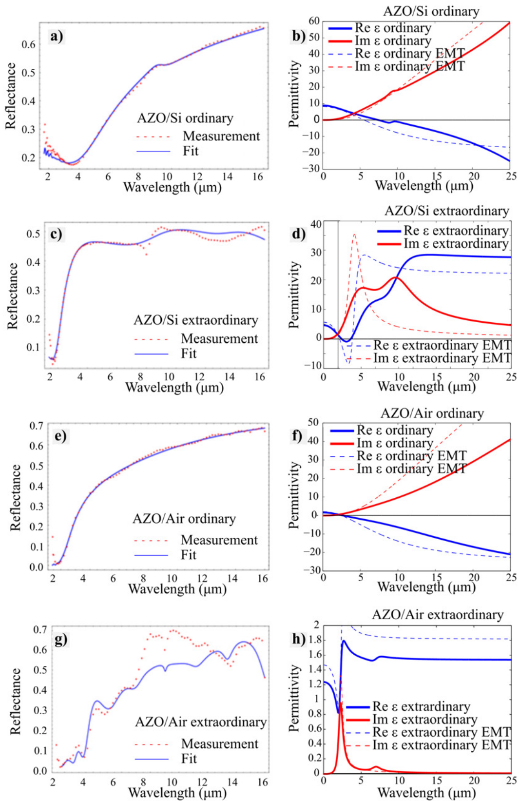
Figure 6.6: FTIR measured and fitted reflection spectra and corresponding retrieved permittivities, together with EMT derived dielectric functions. a) and b) AZO/Si ordinary. c) and d) AZO/Si extraordinary. e) and f) AZO/Air ordinary. g) and h) AZO/Air extraordinary.
