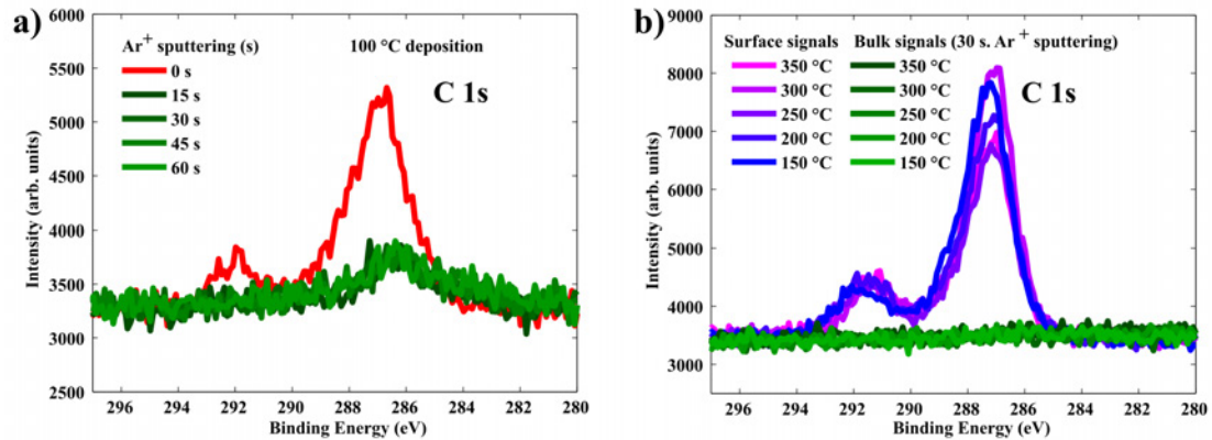
Figure 2.5: High resolution XPS measurements of carbon C 1s . a) The film grown at 100\text{ }^\circ\text{C} contains small amount (approx. At 1%) of carbon due to an incomplete reaction. b) Films grown at higher temperatures show no carbon after their surfaces have been cleaned by Ar^+ ions.
