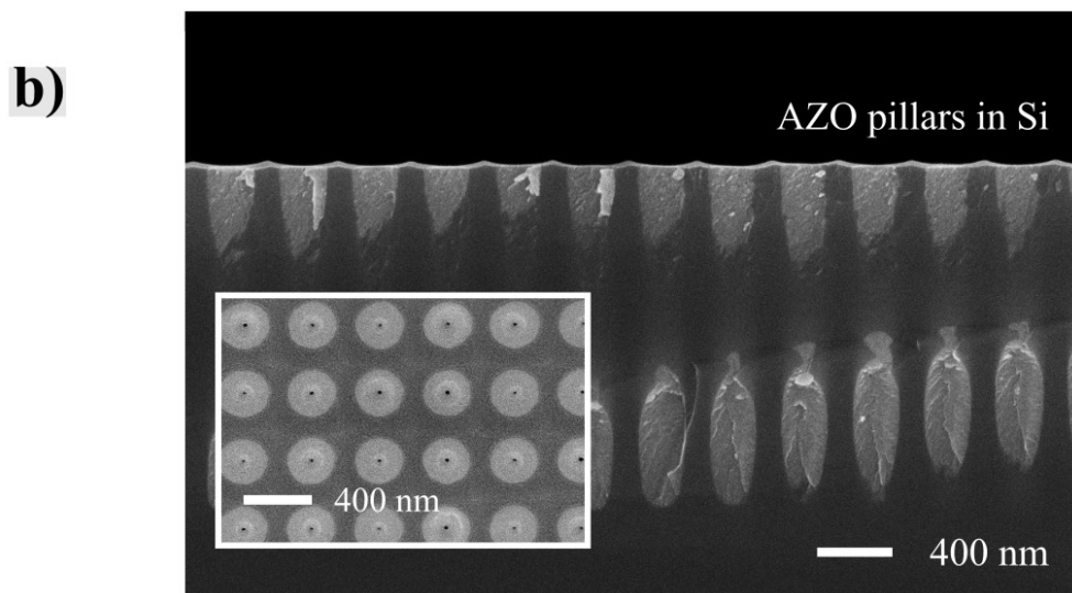
Figure 6.16: AZO/Si pillars HMM. a) Permittivity determined by EMT. At a wavelength higher than \lambda = 6.02\mu\text{m} the structure becomes the Type I hyperbolic. b) SEM image of sample cross-section. The inset shows the pillars from the top.
