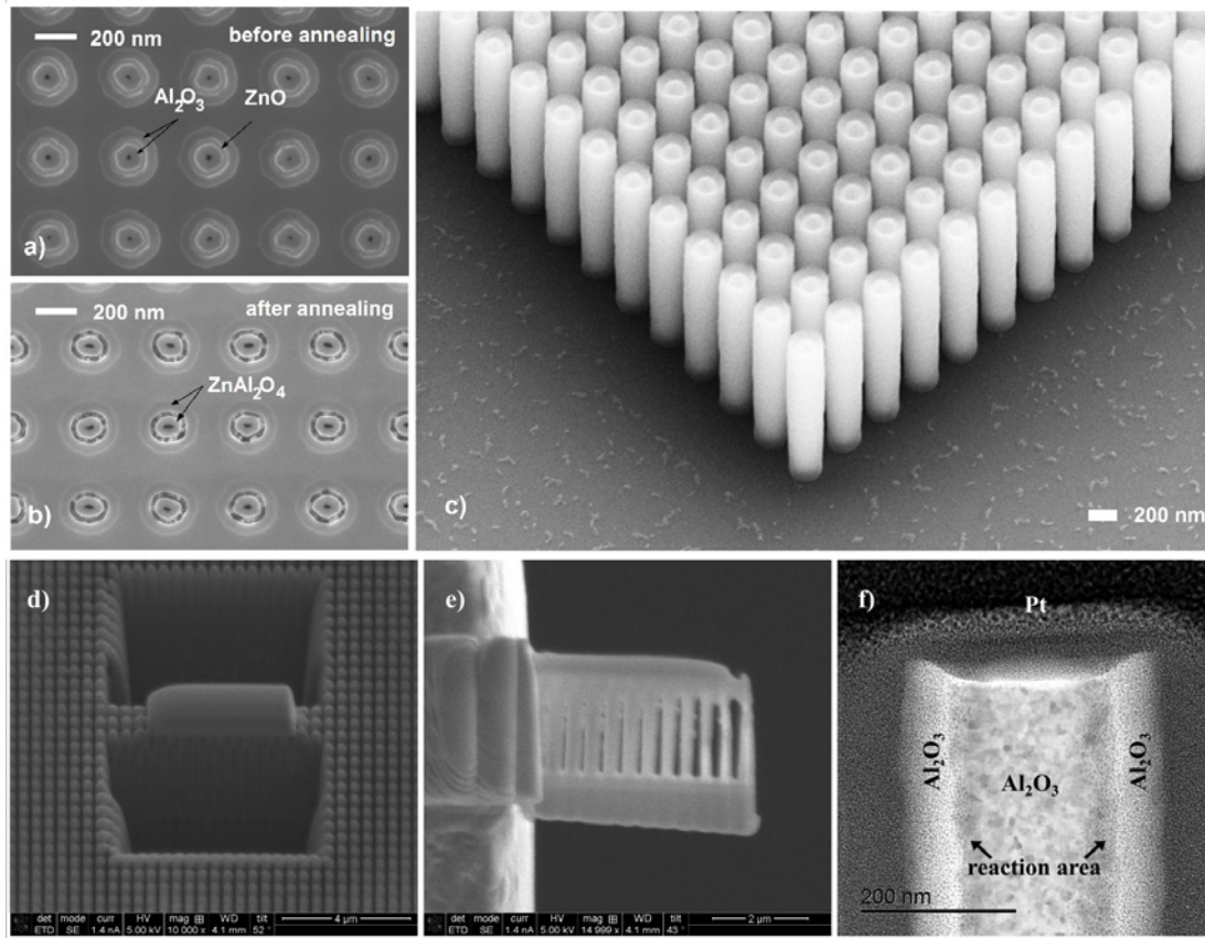
Figure 7.3: SEM images. a) ALD deposition of initial Al_2O_3 and ZnO coatings. b) Temperature induced Kirkendall effect and the formation of ZnAl_2O_4 hollow coaxial pillars. c) Final structure after selective silicon removal. d) Milling the sample using FIB in order to extract the lamella with pillars. e) Fabricated TEM sample, side view. f) High resolution TEM image of a single annealed pillar.
