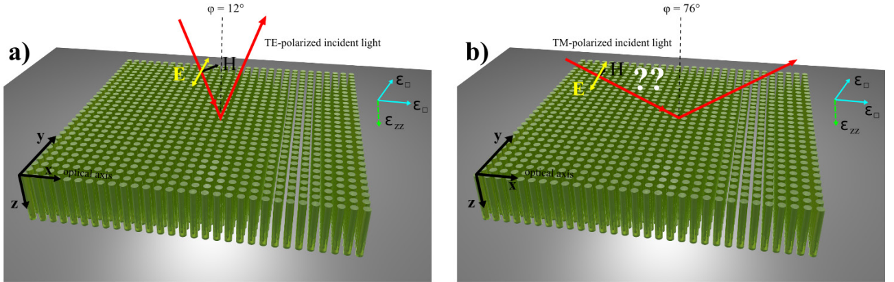
Figure 6.14: Configuration of AZO pillars HMM. a) \mathbf{E} field of incident TE-polarized light, is parallel to the sample surface. Configuration is suitable for recovery of ordinary permittivity \varepsilon_o . b) In order to retrieve extraordinary dielectric function \varepsilon_e , \mathbf{E} field of incident light must be aligned along the pillar direction. If TM-polarized light is incident on the sample with angle of 76^\circ , there are still polarization mixture in the reflection signal, which prohibits the experimental evaluation of extraordinary component \varepsilon_e .
