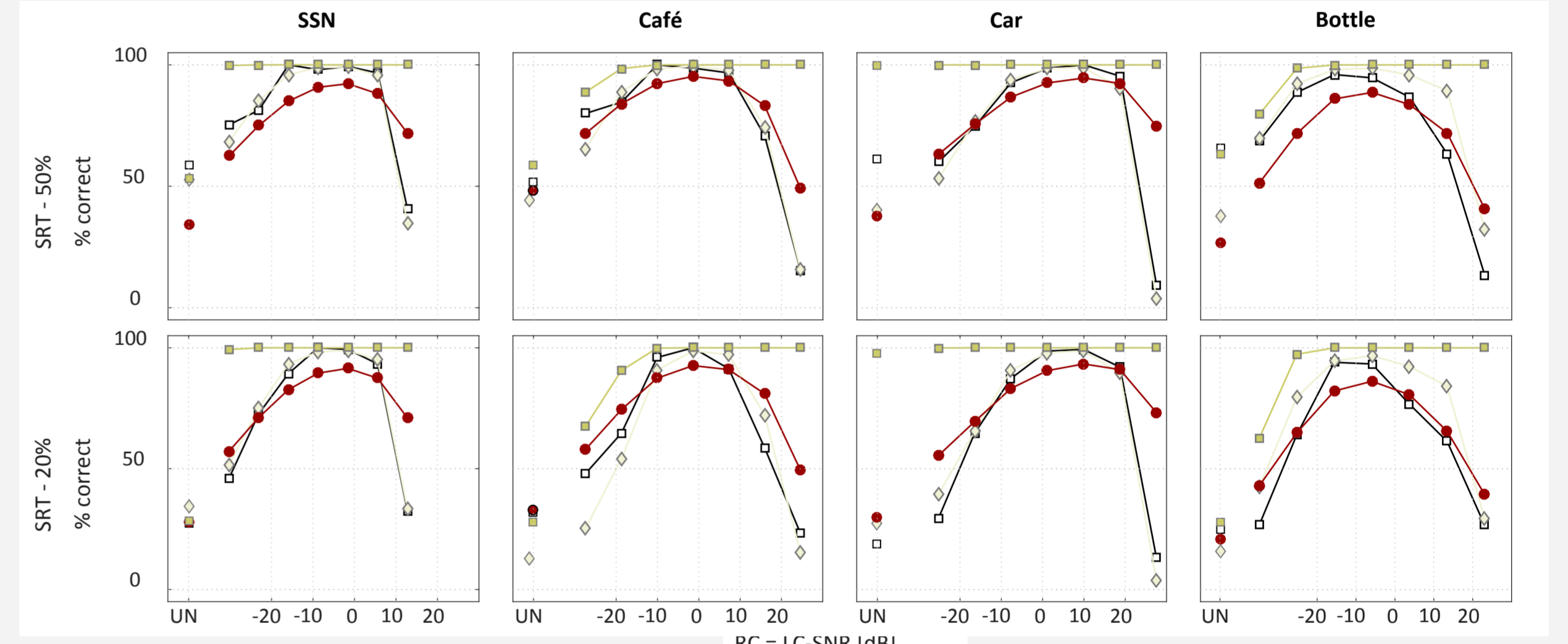
Fig 6. Intelligibility scores for IBM processed speech with four different interferers (columns) and two SNRs (rows). Human data from [2]. mr-sEPSM: \rho = 0.39 STOI: \rho = 0.94 sEPSM corr : \rho = 0.79
