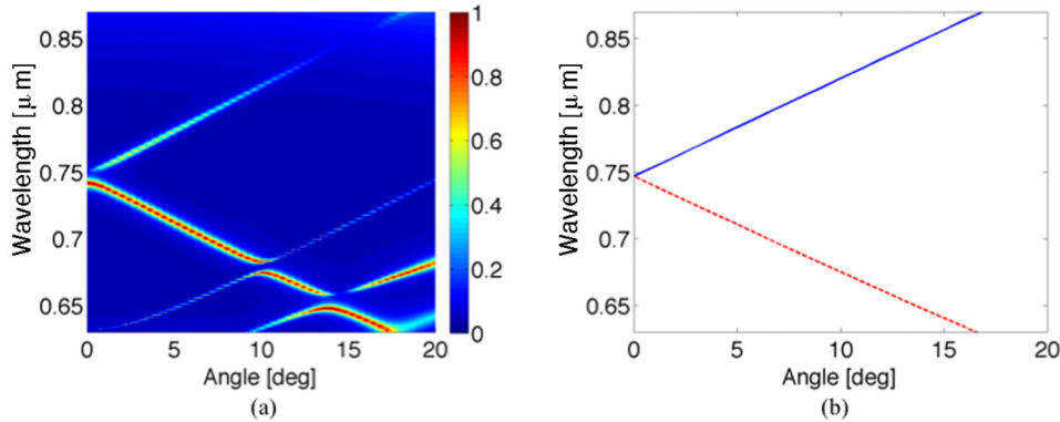
Fig. 5. (a) Angular dependence of the absorption when the incident angle \theta is varied in the range 0^\circ - 20^\circ (the \text{Ta}_2\text{O}_5 slab thickness t_{\text{Ta}_2\text{O}_5} , the periodicity p , the PMMA width w_{PMMA} and the PMMA thickness t_{PMMA} are equal to 100 nm, 470 nm, 305 nm ( w_{PMMA} = 0.65p ) and 650 nm, respectively). (b) Guided resonance mode wavelength dispersion curve versus the angle of incidence for m = 1 (blue solid curve) and m = -1 (red dashed curve), respectively.
