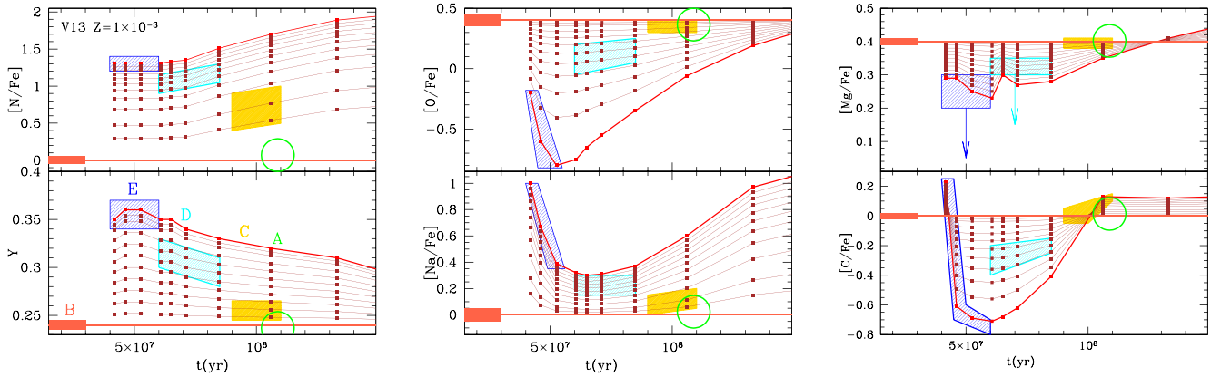
Figure 3. Each panel shows the average abundance of nitrogen (top left), helium (bottom left), oxygen (top centre), sodium (bottom centre), magnesium (top right) and carbon (bottom right) versus time in the ejecta of massive AGB stars having Z = 10^{-3} (Ventura et al. 2013). The yield for each initial mass (8, 7.5, 7, 6.5, 6.3, 6.0, 5.5, 5.0, 4.5 M_{\odot} , from left to right) is shown by dots. The abundances of oxygen at t < 7 \times 10^7 yr have been adjusted as explained in the text. The pure ejecta abundances are shown as a red line with squares. The initial abundances in the AGB stars are represented by the horizontal red lines without dots. Abundances in diluted matter are shown by the brown lines with squares. Starting from the initial FG abundance lines, the AGB gas percentage in each curve is 0.05, 0.1, 0.2, 0.3, . . . , 0.9. In these planes, we show our guess for the location of the five populations defined by Milone et al. (2015a) for the cluster NGC 2808: (1) B (red) is the FG population, having the initial gas abundances (red rectangles, stars born at t = 0 ); (2) E is the most extreme SG, born from pure AGB ejecta, defined by the blue rectangles; (3) D is the ‘intermediate’ SG, in which the AGB ejecta constitute 40–60 per cent of the forming gas (cyan regions); (4) C, the new population discovered in Milone et al. (2015a), with normal helium and high nitrogen: this is obtained by very strong dilution of the AGB ejecta which already have a strong effect of 3DU, with CNO enhancement; (5) A, the small population at the red of all other sequences, is here identified with a remnant SF, mostly from FG gas contaminated by the ejecta of one SN Ia (green circle). The Mg boxes for population E and D (blue and cyan) in the bottom-right panel show with arrows the observed location in the data by Carretta (2015), \sim 0.15 dex lower than the models. As explained in the text, a lower mass-loss rate would provide the correct result, but it would reduce the sodium abundances.
