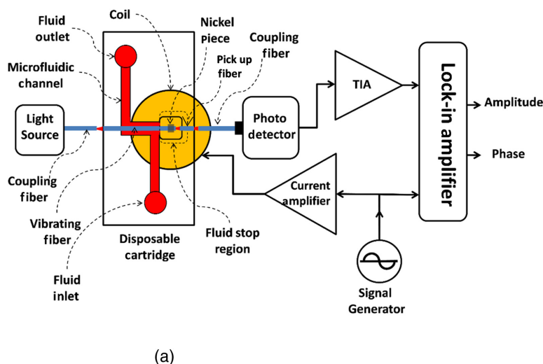
Fig. 1 (a) Schematic of the measurement setup. Optical fiber is actuated remotely by an electrocoil. Optical signal is collected through a silicon photodetector. Amplitude and phase of the signal are monitored by a lock-in amplifier. (b) A photo of the measurement setup with cartridge. Blood sample is inserted into the microfluidic channel through an inlet. Blood flows with capillary motion into the cartridge.
