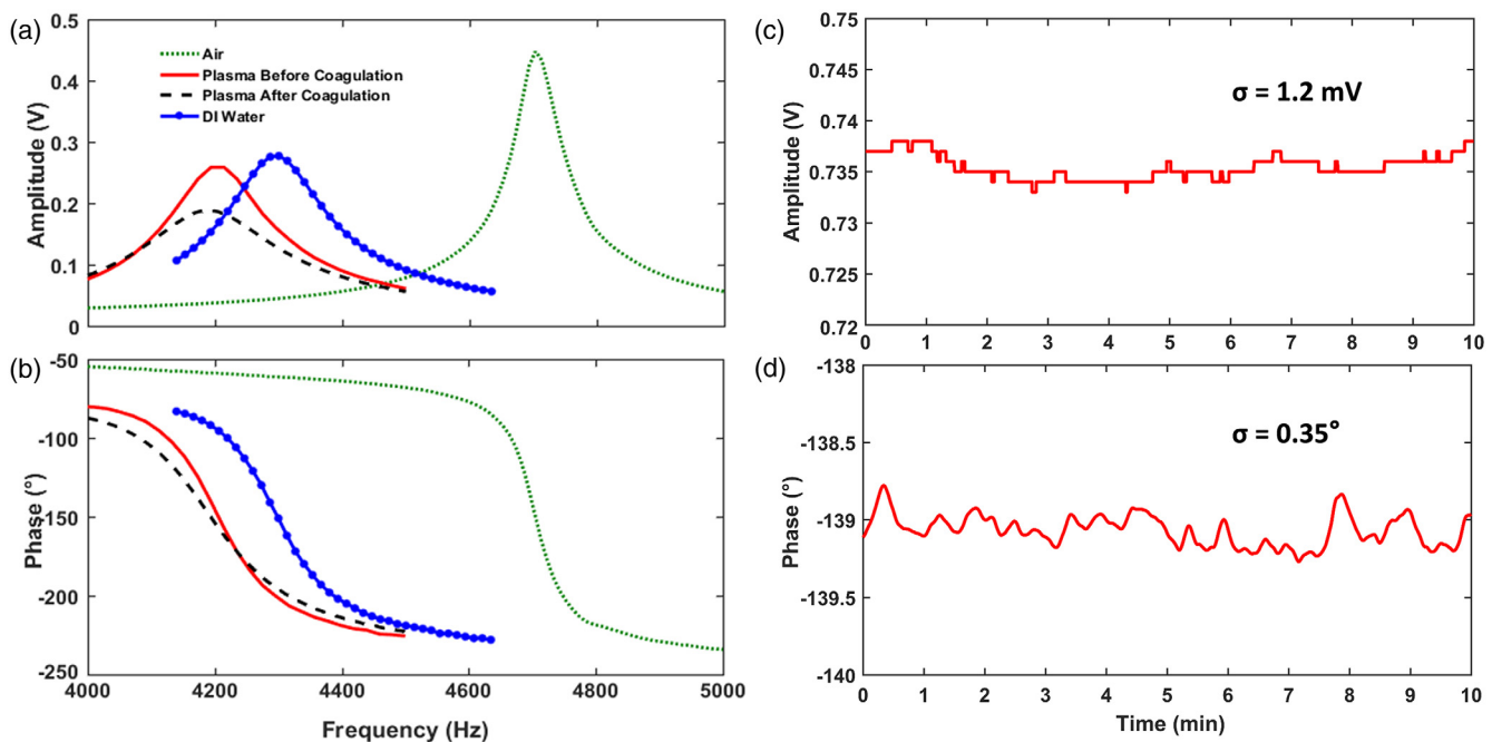
Fig. 3 Frequency response of the system to air, distilled water, uncoagulated blood plasma, and blood plasma after coagulation. Amplitude and phase change are shown in (a) and (b), respectively. (c) Amplitude and (d) phase stability of the sensor in distilled water for 10 min. Amplitude has a standard deviation of 1.2 mV, and phase has a standard deviation of 0.35 deg.
