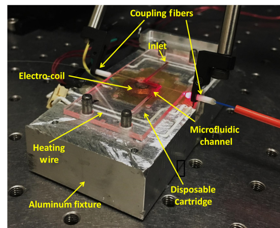
Fig. 1 (a) Schematic of the measurement setup. Optical fiber is actuated remotely by an electrocoil. Optical signal is collected through a silicon photodetector. Amplitude and phase of the signal are monitored by a lock-in amplifier. (b) A photo of the measurement setup with cartridge. Blood sample is inserted into the microfluidic channel through an inlet. Blood flows with capillary motion into the cartridge.
