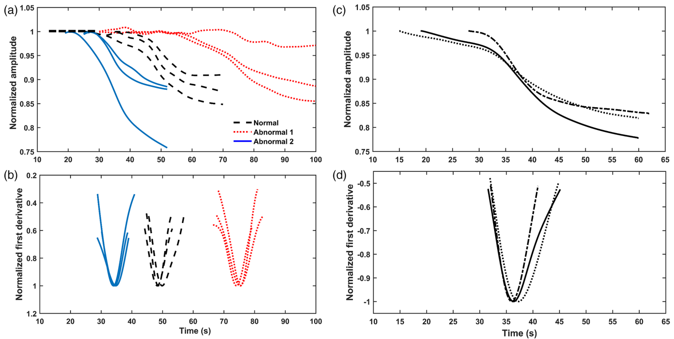
Fig. 5 (a) aPTT tests with normal, abnormal 1, and abnormal 2 control plasmas. Each test was repeated three times with the same control plasma samples but different cartridges. (b) First derivatives of control plasma results show the local minima. (c) aPTT tests were repeated for human whole blood sample three times with the same sample but different cartridges. (d) First derivatives of whole blood results show the local minima. \sigma = 0.76 s and RSD% = 2.
