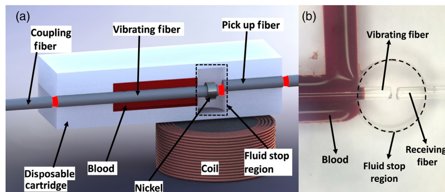
Fig. 2 (a) A cross sectional 3-D sketch of the cartridge with electrocoil. Blood inlet and outlet are not shown. Blood does not get into the fluid stop region due to capillary force at the boundary. (b) Top view microscope picture of the fluid stop region with blood in the microfluidic channel. Note that the tip of the fiber is free to move; there is no physical barrier. Also note that the Ni piece is not attached to the fiber cantilever shown here since it is not a functional cartridge but fabricated only for fluid stop illustration.
