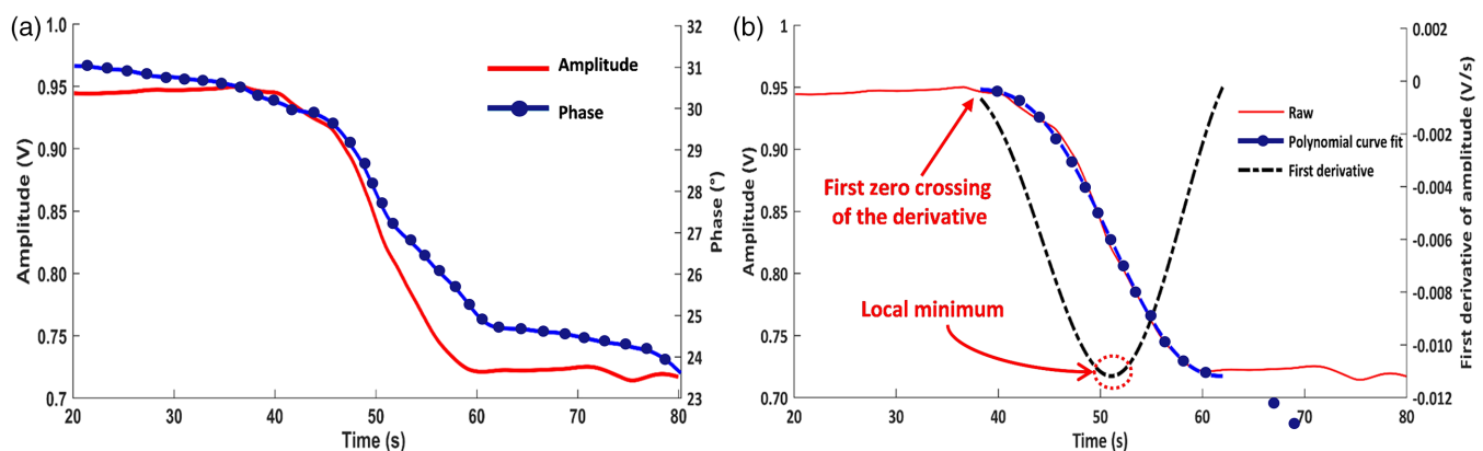
Fig. 4 (a) Amplitude and phase change during coagulation of abnormal 1 control plasma. (b) Polynomial fit to amplitude and its first derivative. Time of local minimum of the derivative is reported as coagulation times. First zero crossing of the derivative indicates the clot formation time.
