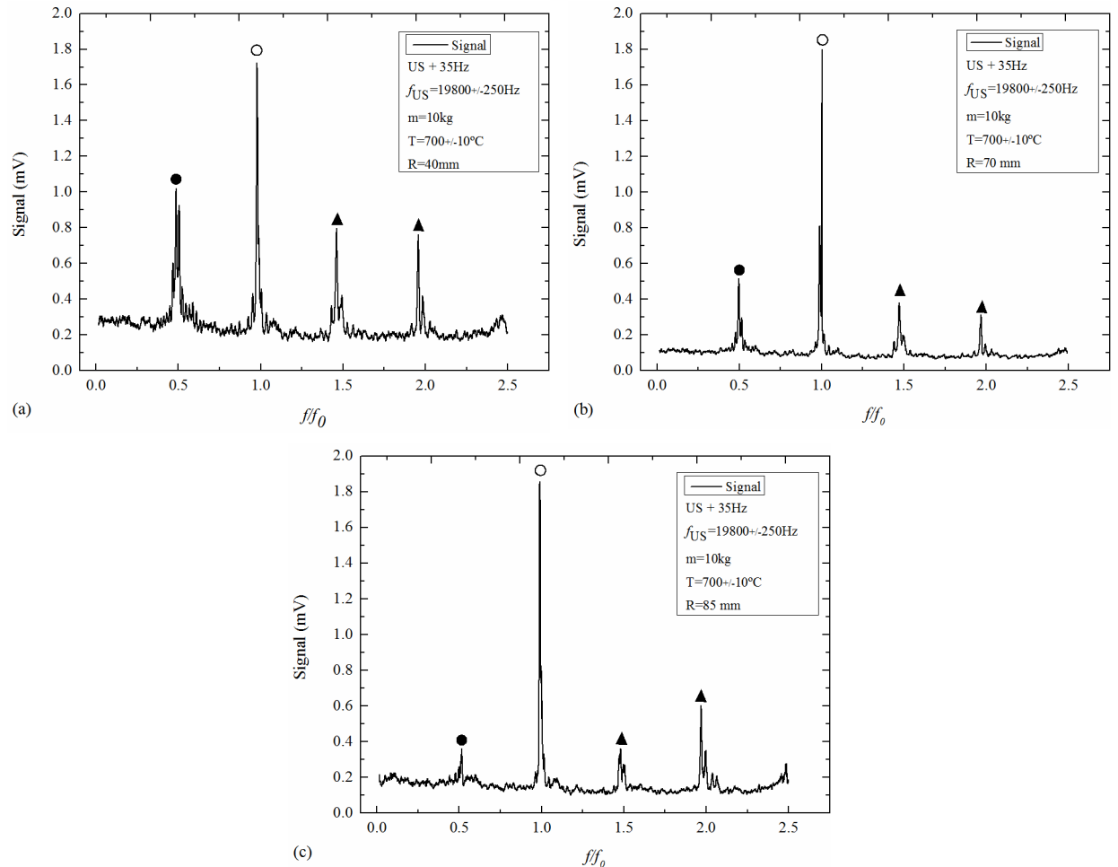
Fig. 8. FFT spectral levels of harmonics ( \circ ), sub ( \bullet ) and ultra-harmonics ( \blacktriangle ) of acquired sound pressure waveform at different distances from the acoustic radiator, during the combined effect degassing process: (a) R=40 mm - distances from the acoustic radiator; (b) R=70 mm - distances from the acoustic radiator. (c) R=85 mm - distances from the acoustic radiator
