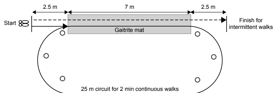
Figure 3 This figure depicts the laboratory setup for testing continuous and intermittent walks.
