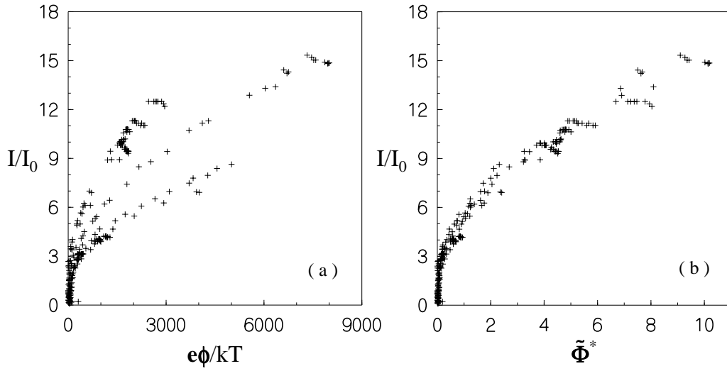
Fig. 1. – I - V characteristics derived from TSS-1R data [4]: (a) normalized current is plotted vs. e\Phi/KT_e ; (b) normalized current is plotted vs. the parameter \tilde{\Phi}^* defined in eq. (35).
