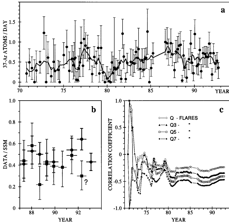
Fig. 1. – a) Homestake neutrino data with error bars, and 5-point running-averaged values (solid line): from run No. 18 to No. 126; b) comparison between Kamiokande (circles) and Homestake (squares) neutrino data averaged over the same time intervals: the last point of Homestake data (with a question mark) contains two runs that do not have still definitive values; c) time evolution of correlation coefficients of solar flares with 3-, 5- and 7-point running averages of Homestake neutrino data.
