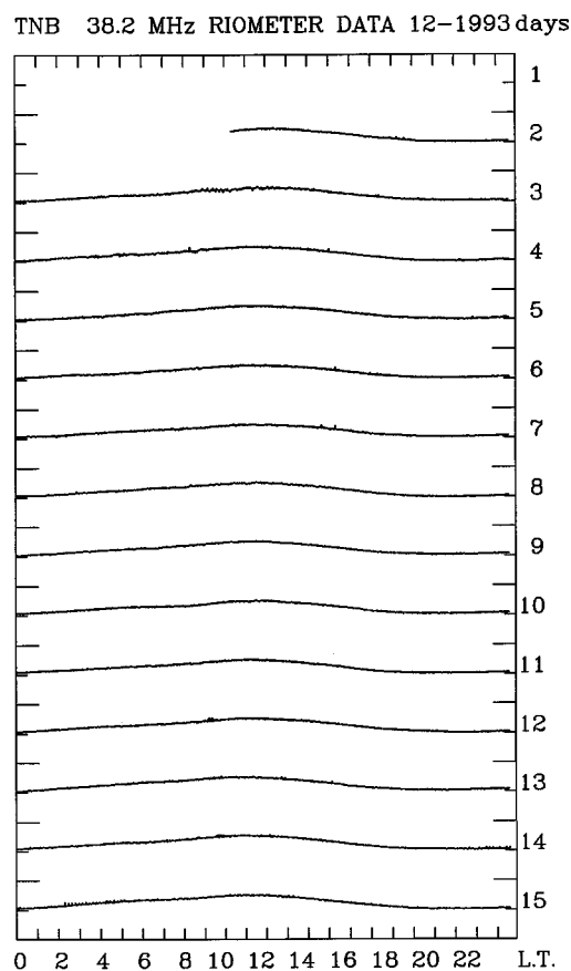
Fig. 2. – Daily behaviour of cosmic noise (arbitrary units) at 38.2 MHz as measured at Terra Nova Bay (Antarctica) for the first half month of December 1993.
