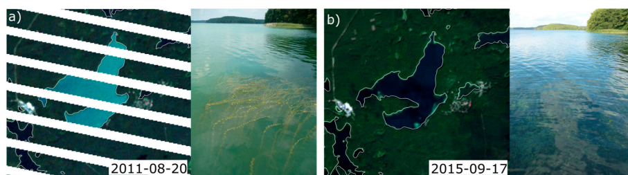
Figure 8. Two quasi-true color Landsat RGB of Stechlinsee with photos showing the water surface taken from a boat: (a) August 2011, showing the lake with calcite precipitation; and (b) September 2015, with clear water. The photos were taken: (a) two days before; and (b) nine days after the Landsat acquisition.
