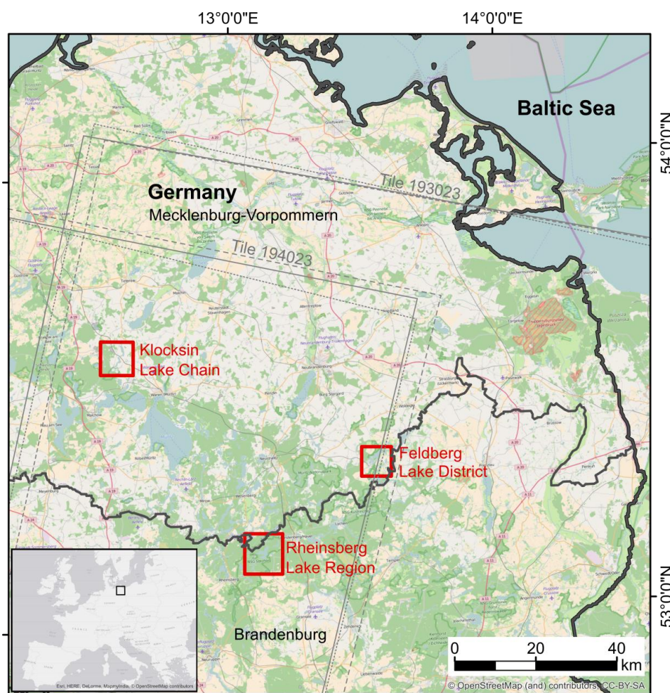
Figure 1. Study area with three selected regions: Feldberg Lake District, the Klocksinn Lake Chain, and Rheinsberg Lake Region. The gray lines illustrate the Landsat footprints of the acquisition tiles 193023 and 194023. The gray dashed line shows the footprint of Landsat 5, the solid gray line shows the footprint of Landsat 7, the dotted gray line the footprint of Landsat 8.
