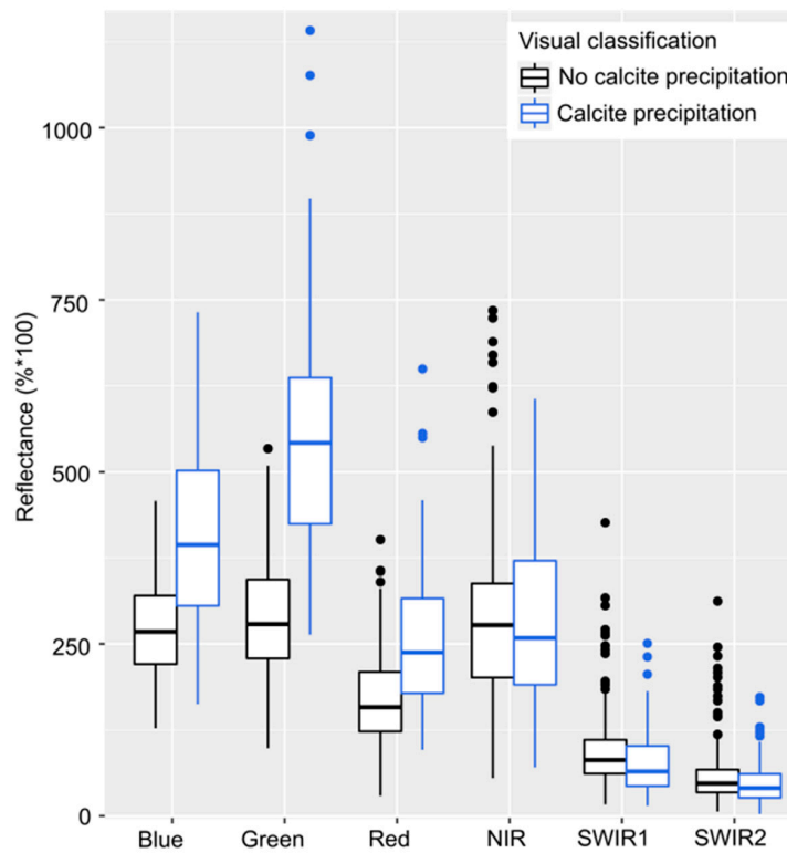
Figure 11. Reflectance values in all spectral bands of Breiter Luzin, Schmaler Luzin and Feldberger Haussee of good quality images. All three lakes are visually classified as turquoise (calcite precipitation) or dark (no calcite precipitation).
